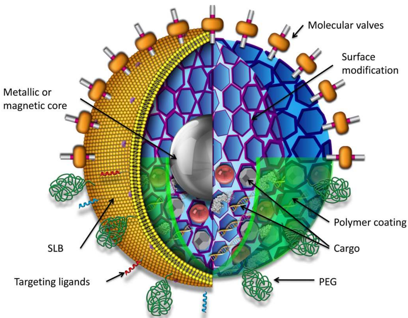
FIGURE 1. Schematic of multifunctional mesoporous silica nanoparticle showing possible core/shell design, surface modifications, and multiple types of cargos. cargos
