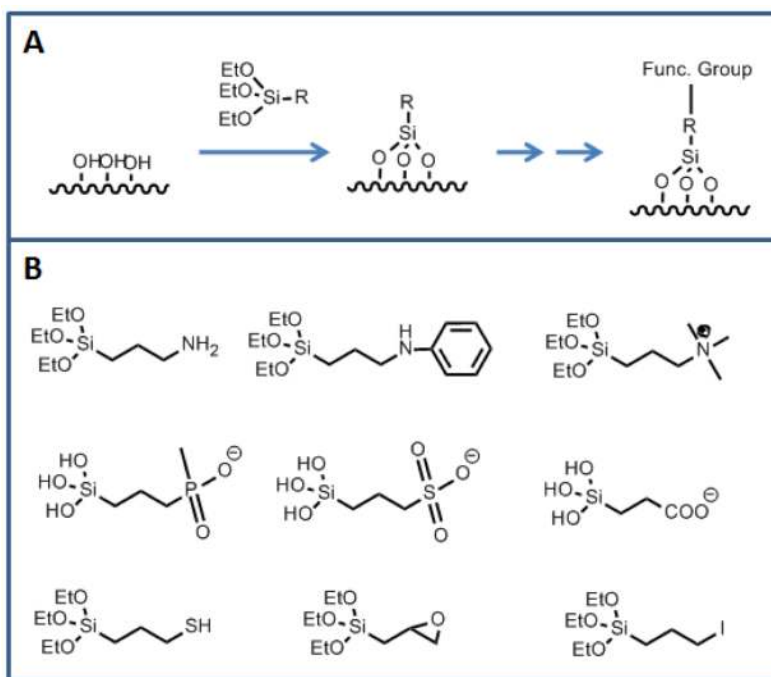
FIGURE 3. (a) Schematic showing reaction of surface silanol groups with an alkoxy silane linker to introduce functionality. (b) Various linkers to attach bio-molecules or to change the surface properties.
