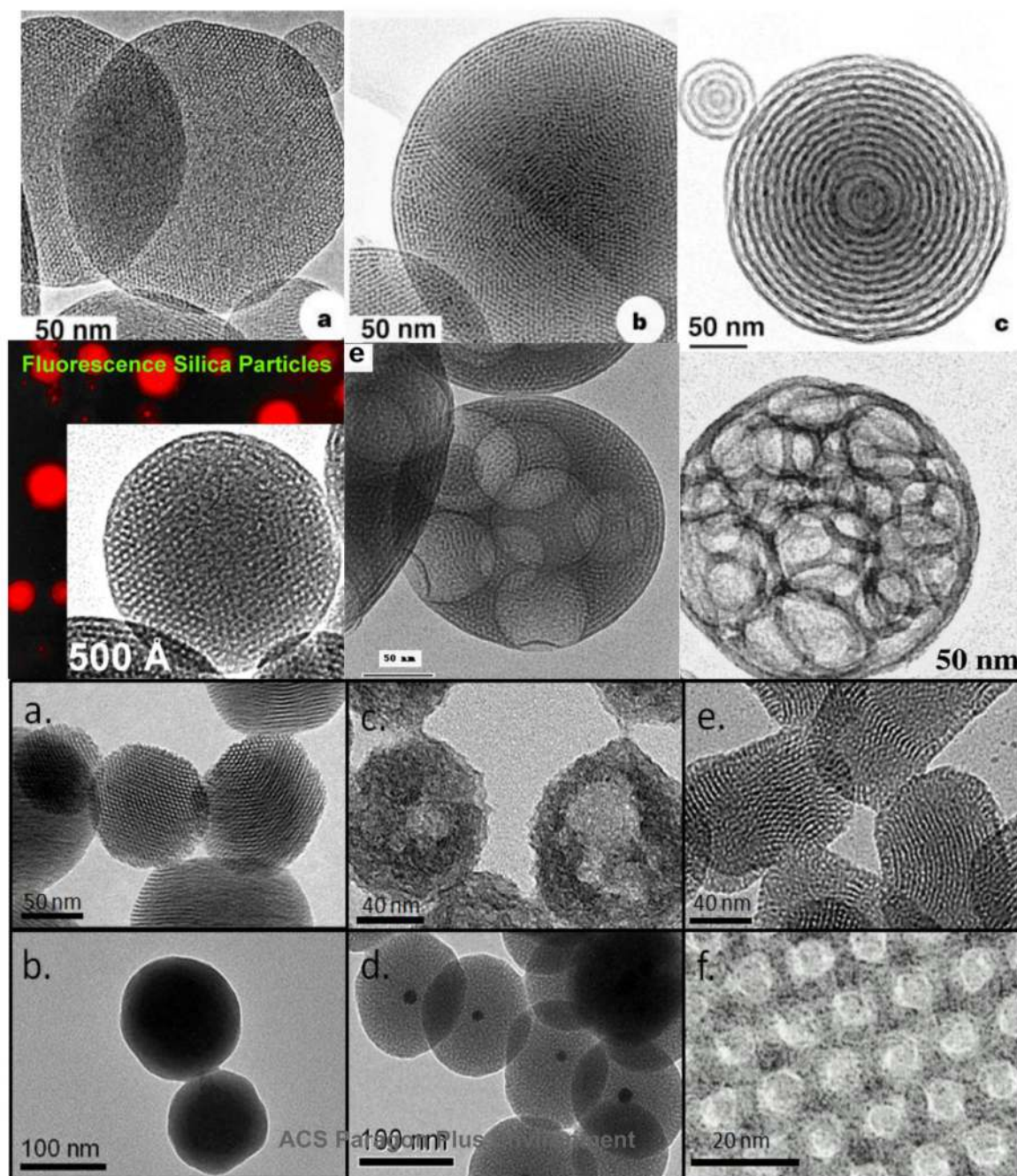
FIGURE 2. Gallery of mesoporous silica nanoparticles. Particles in a, b, c, and d are formed by EISA. Lower panel are solution prepared MSNPs. 7
