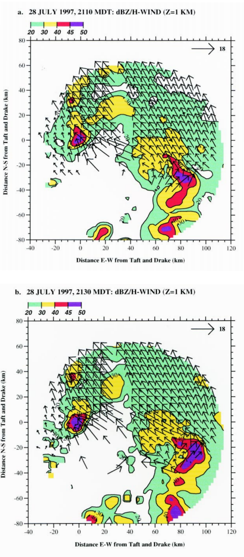
FIG. 12. Dual-Doppler-derived horizontal wind vectors ( \text{m s}^{-1} ) and radar reflectivity (shaded) for the 1-km height level at (a) 2110 MDT 28 July 1997 and (b) 2130 MDT 28 July 1997. Grid origin as in Fig. 9. Vector scale ( \text{m s}^{-1} ) is indicated in the upper-right corner.
