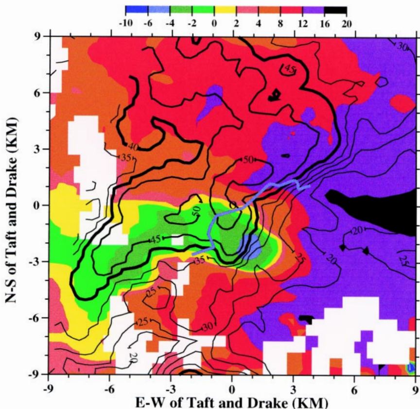
FIG. 10. CSU-CHILL 2115 MDT 28 July 1997: radial wind velocity (shaded in \text{m s}^{-1} ) at 300-m AGL and radar reflectivity (1.2 km AGL) contoured every 5 dBZ, beginning at 20 dBZ. The CSU-CHILL radar is located at an azimuth of 116° and ~40–45 km from the origin (as in Fig. 9). Warm colors indicate outbound radial velocities (~easterly, southeasterly), cool colors indicate inbound (~westerly) radial velocities. A portion of Spring Creek is also indicated by the bold blue line running through the origin. Note that wind data are missing on the west side of the figure where elevated terrain is located.
