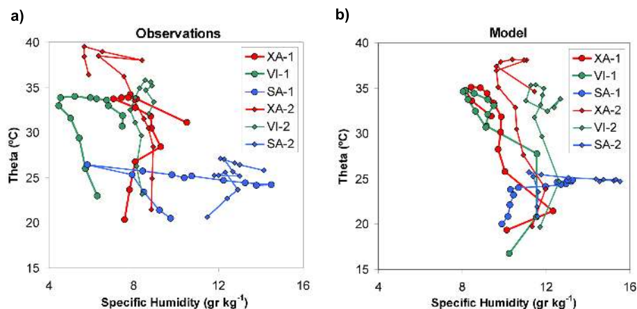
Fig. 5. Scatter plot of virtual potential temperature vs. specific humidity hourly data at weather stations XA (red), VI (green) and SA (blue) observed (a) and modeled (b), for the daytime period of 06:00 to 18:00 UTC on 1 July (–1) and 2 July (–2).
