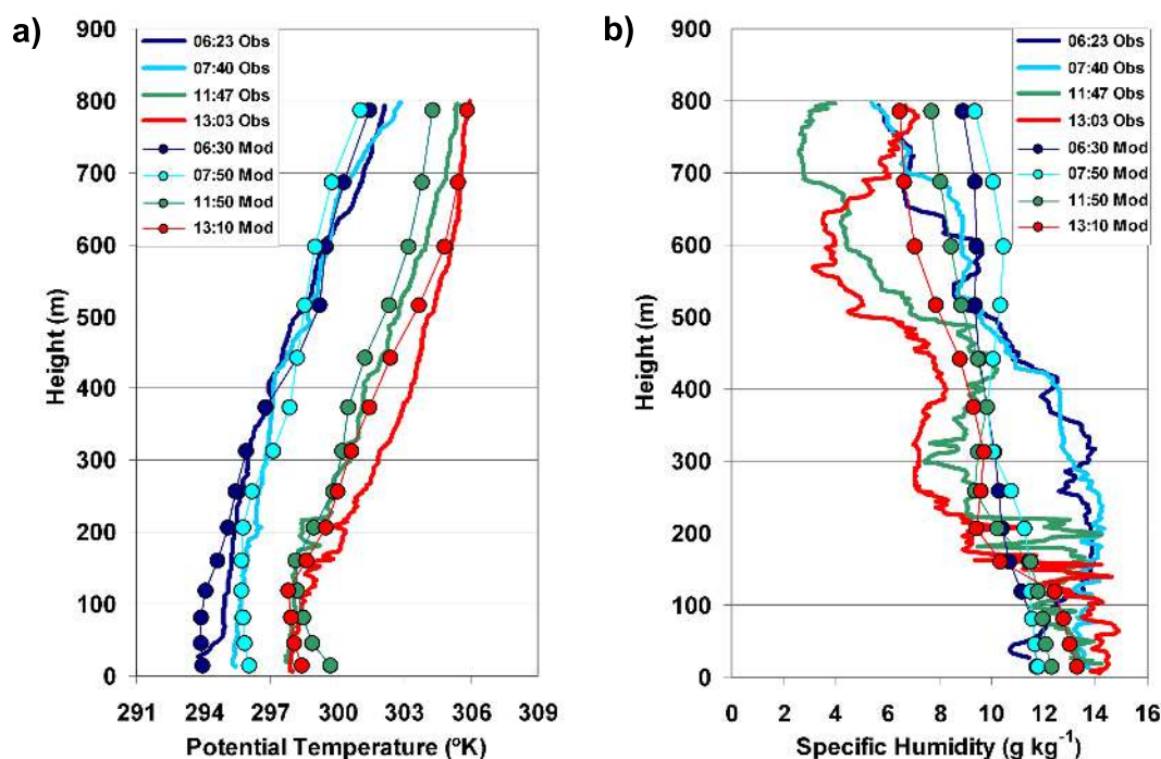
Fig. 9. Observed (Obs) and modeled (Mod) vertical profiles of potential temperature (left) and q (right) over the rice paddy fields at the aircraft campaign location (marked with P in Fig. 1b) at different times on 2 July.
