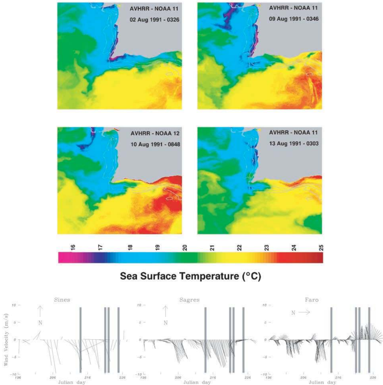
Figure 7. Set of thermal infrared NOAA-AVHRR images for the first half of August 1991, when the Cape São Vicente filament was developing. Images were processed for sea surface temperature. The 100, 200, and 500 m depth contours are overlaid to the images. Stick vector time series of the wind field measured at Sines, Sagres, and Faro from 15 July till 15 August are also displayed. Wind vector ordinate represents the alongshore wind component. Image dates are indicated in the stick diagrams (2 August, day 214; 9 August, day 221; 10 August, day 222; and 13 August, day 225).
