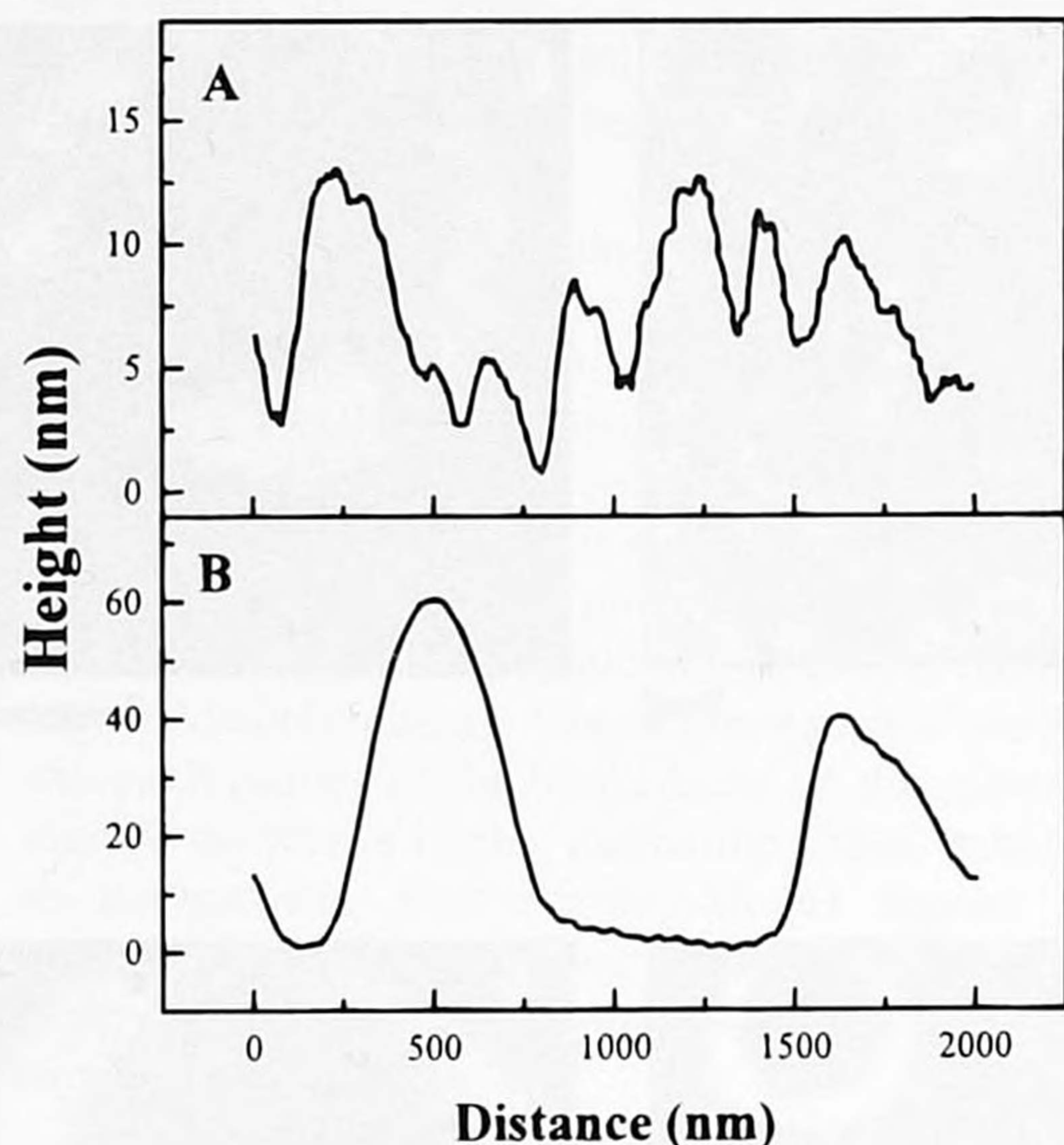
Figure 10. Selected topographic line scans on a 2 \mu\text{m} length scale. (A, B) Line scans taken from parts F and I of Figure 7, respectively.
