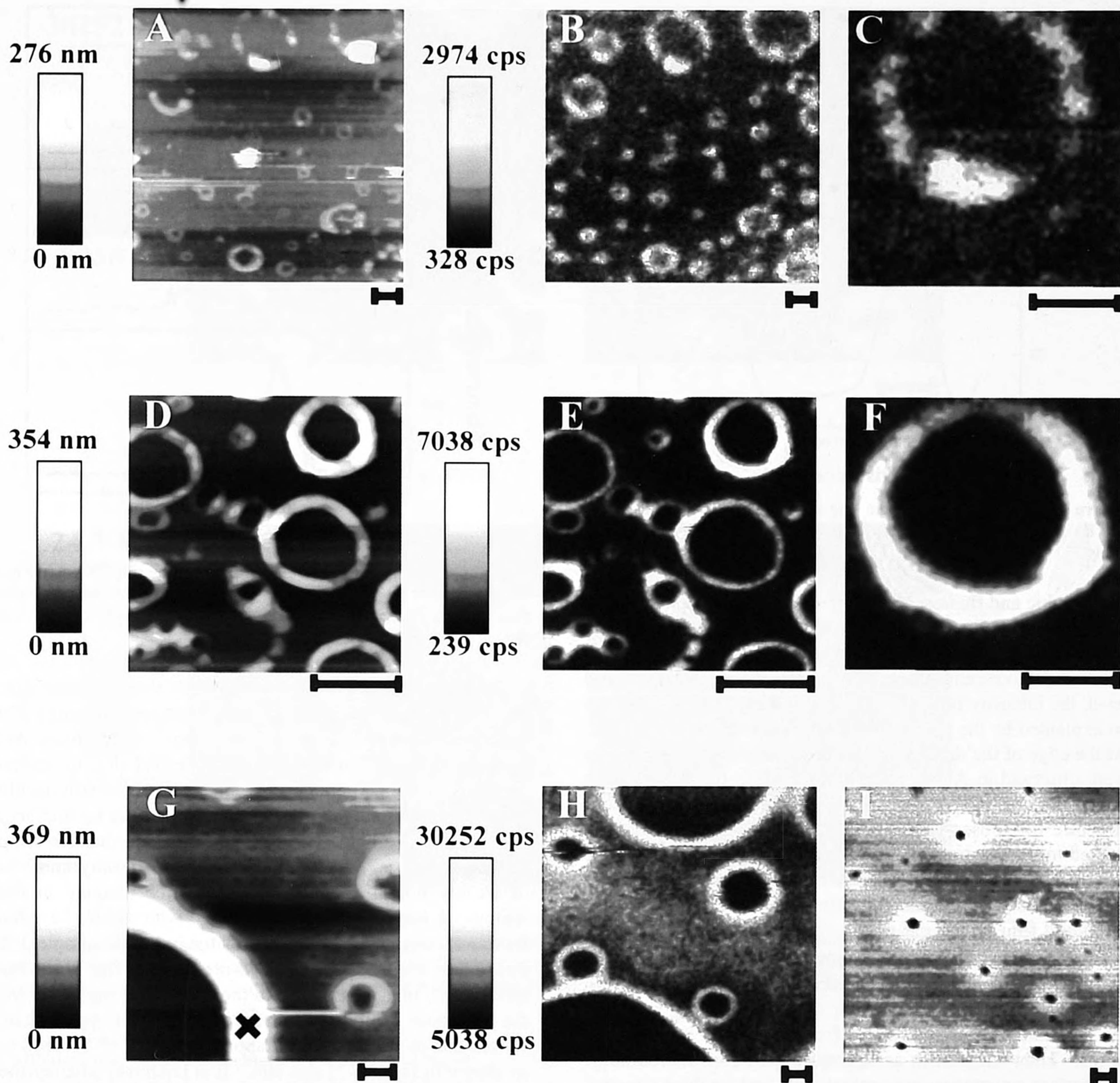
Figure 9. Near-field and topographic images of evaporated films of PtP/CHCl 3 solutions on glass. The black scale bar below each image represents 1 \mu m. (A, B) Topographic and corresponding near-field image taken on a sample prepared by solvent casting of a 2 \times 10^{-7} M solution. (C) Enlarged view of the top middle ring displayed in B. (D, E) Topographic and corresponding near-field image taken on a sample prepared by solvent casting of a 2 \times 10^{-6} M PtP/CHCl 3 solution. (F) Enlarged view of the top right ring displayed in B. (G, H, I) Topographic and near-field images taken on a sample prepared by solvent casting of a 1 \times 10^{-4} M PtP/CHCl 3 solution. H is taken in the middle of the droplet, while I is taken at the edge of the sample. The \times in G indicates the position where spectra were acquired. The color scale beside figure H only applies for I. For I the color scale beside E is valid.
