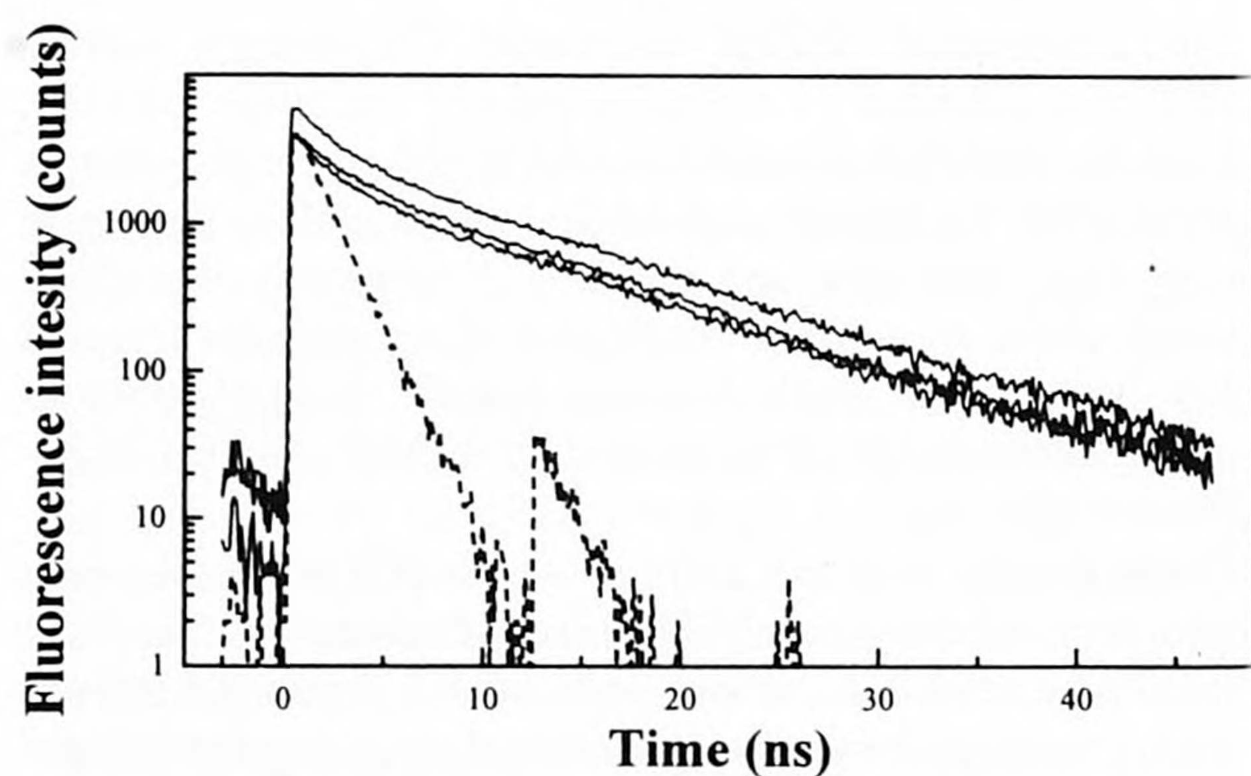
Figure 3. Decay curves obtained by scanning the amorphous material between rings (full line), an isolated ring (bold line), and an aggregate in a ring (thin line). The dotted line is the decay of the reference.
