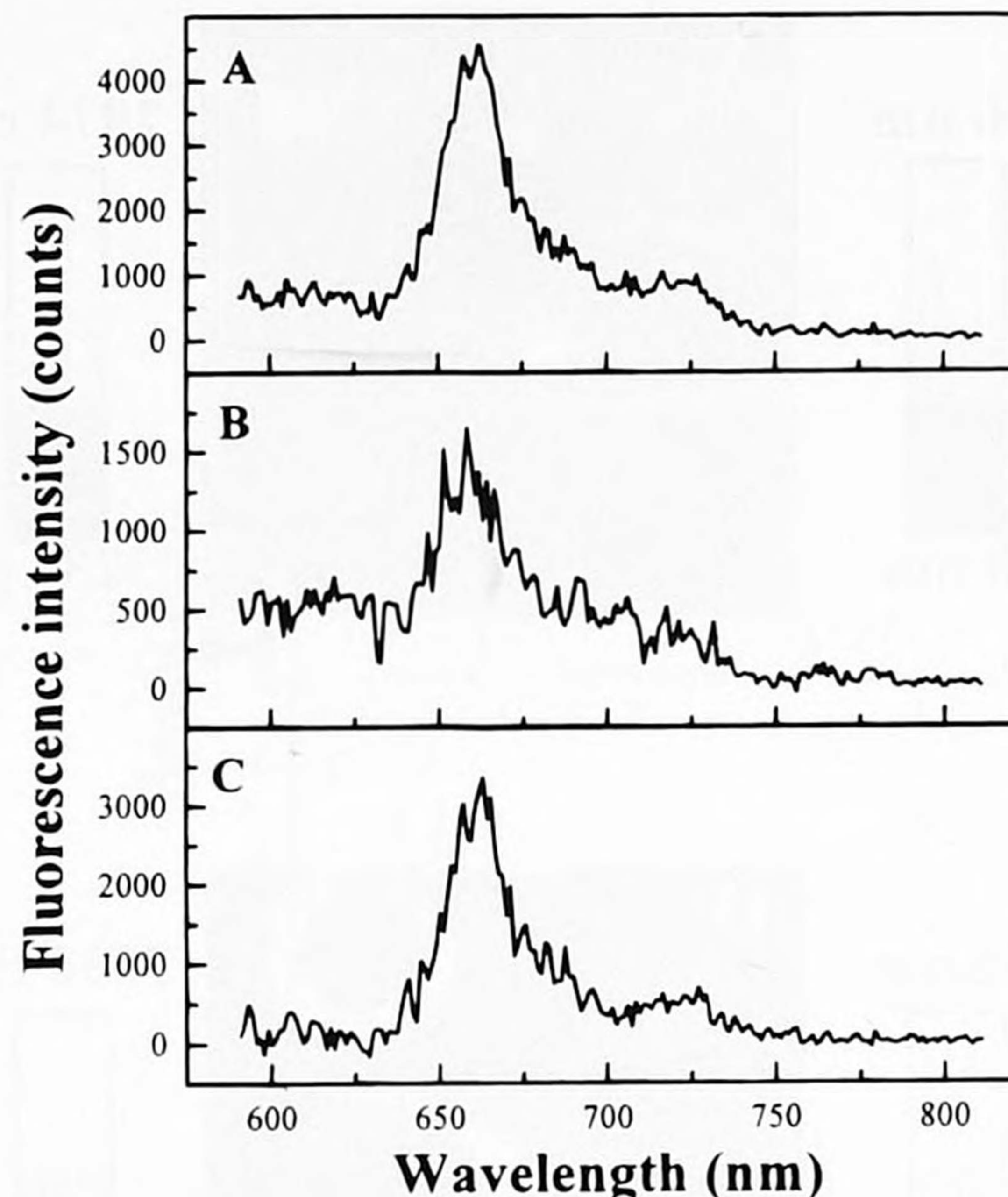
Figure 11. (A) Spectrum taken on the rim of the ring shown in Figure 7C. Acquisition time 60 s. (B) Fourth spectrum in a row with acquisition time of 60 s on the same position. (C) Difference spectrum of A and B.
