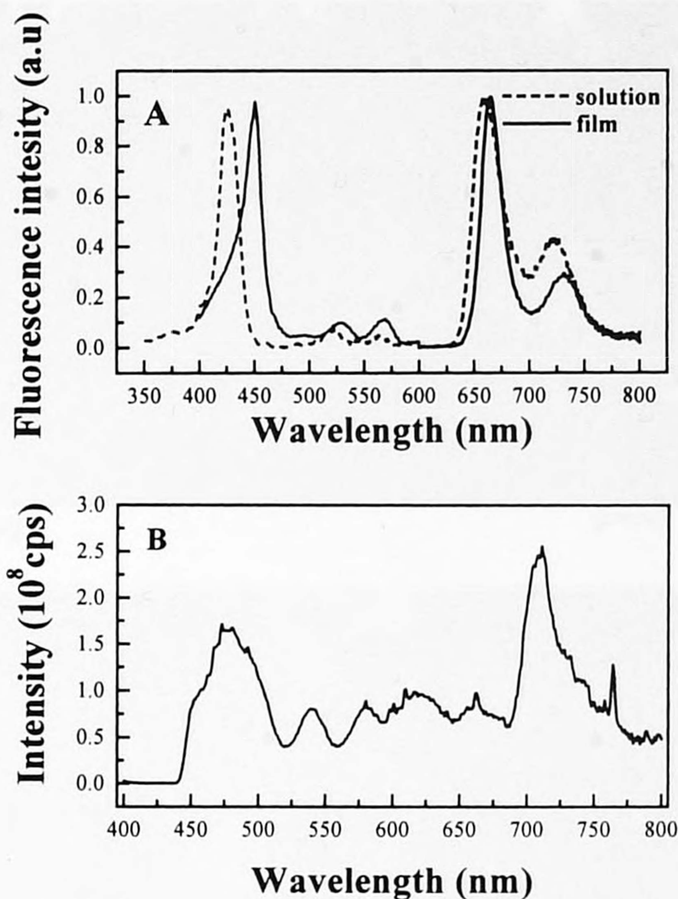
Figure 1. (A) Excitation and emission spectra of PtP deposited on glass (full line) and in \text{CHCl}_3 solution (dotted line); emission spectra taken on a sample prepared by evaporating a 2 \times 10^{-4} M solution in \text{CHCl}_3 . (B) Synchronous scan of a 5 \times 10^{-5} M solution of PtP in \text{CHCl}_3 .
