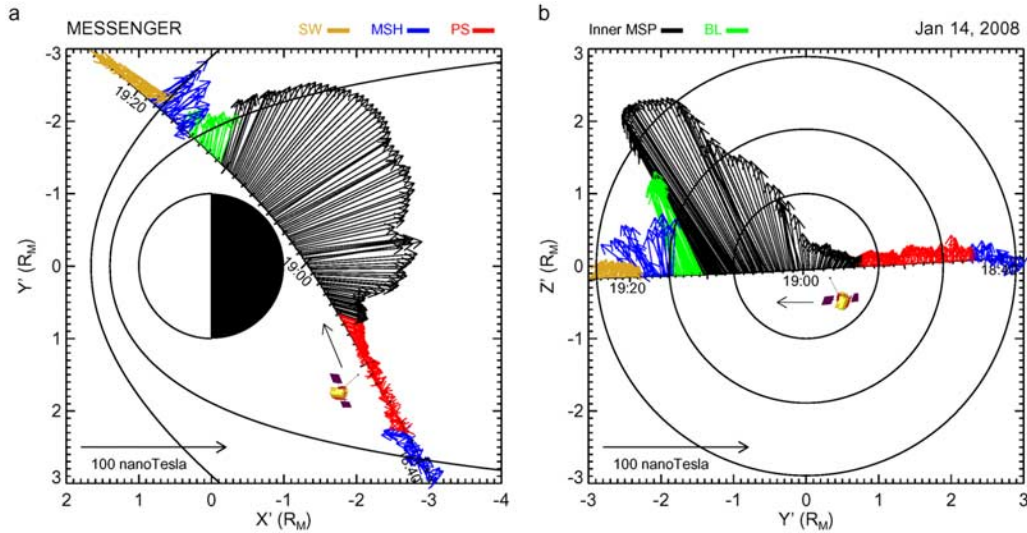
Figure 2. (a) MESSENGER magnetic field vectors (10-s averages) are projected onto the aberrated X_{MSO}-Y_{MSO} plane. (b) Similar display, but for the aberrated Z_{MSO}-Y_{MSO} plane. As indicated, different colors are used to identify the different boundaries and regions of the magnetosphere (SW, solar wind; MSH, magnetosheath; PS, plasma sheet; MSP, magnetosphere; BL, boundary layer). Bow shock and magnetopause model surfaces are also shown.
