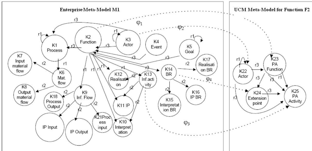
Figure 7. The mapping of Enterprise Meta-Model M1 elements to UCM Meta-Model F2
