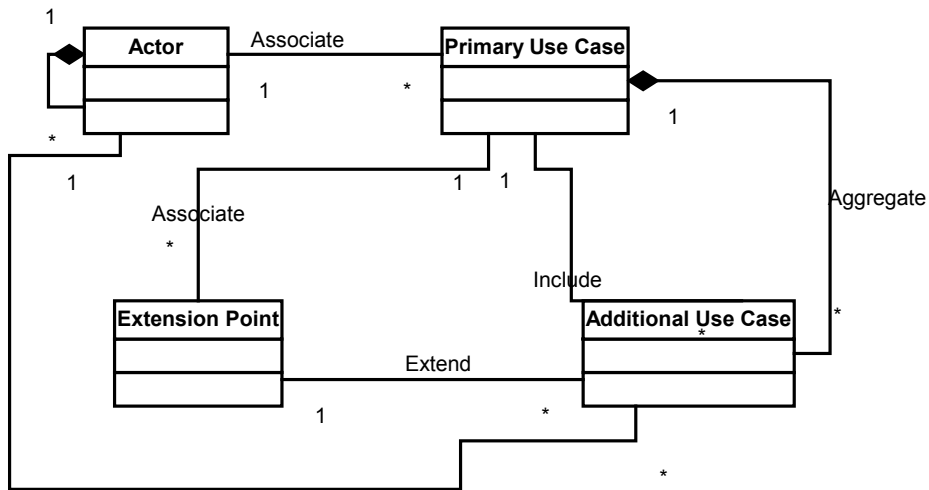
Figure 4. UCM meta-model
