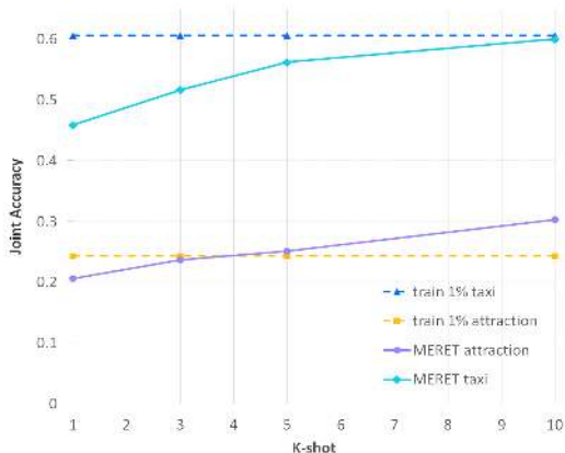
Figure 3: K-shot results of different experimental settings. Performance of our model surpasses training from scratch on attraction domain with K=5 .
