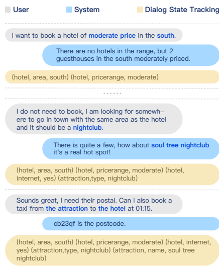
Figure 1: An example of dialogue state tracking process for booking a hotel, looking for an attraction and booking a taxi between them. Each turn contains a user utterance (grey) and a system utterance (blue). The dialogue state tracker (yellow) tracks all the ( domain, slot, value ) until the current turn. Blue color texts indicate mentions of slot values appeared at that turn. Best viewed in color.
