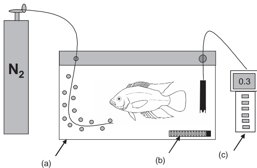
Fig. 2. Set up to analyze \text{MO}_2 and opercular movements of A. crassipinnis and S. aequifasciatus (experiment 2). (a) Pespex aquaria—6 L; (b) Temperature control; (c) Oxygen meter.
