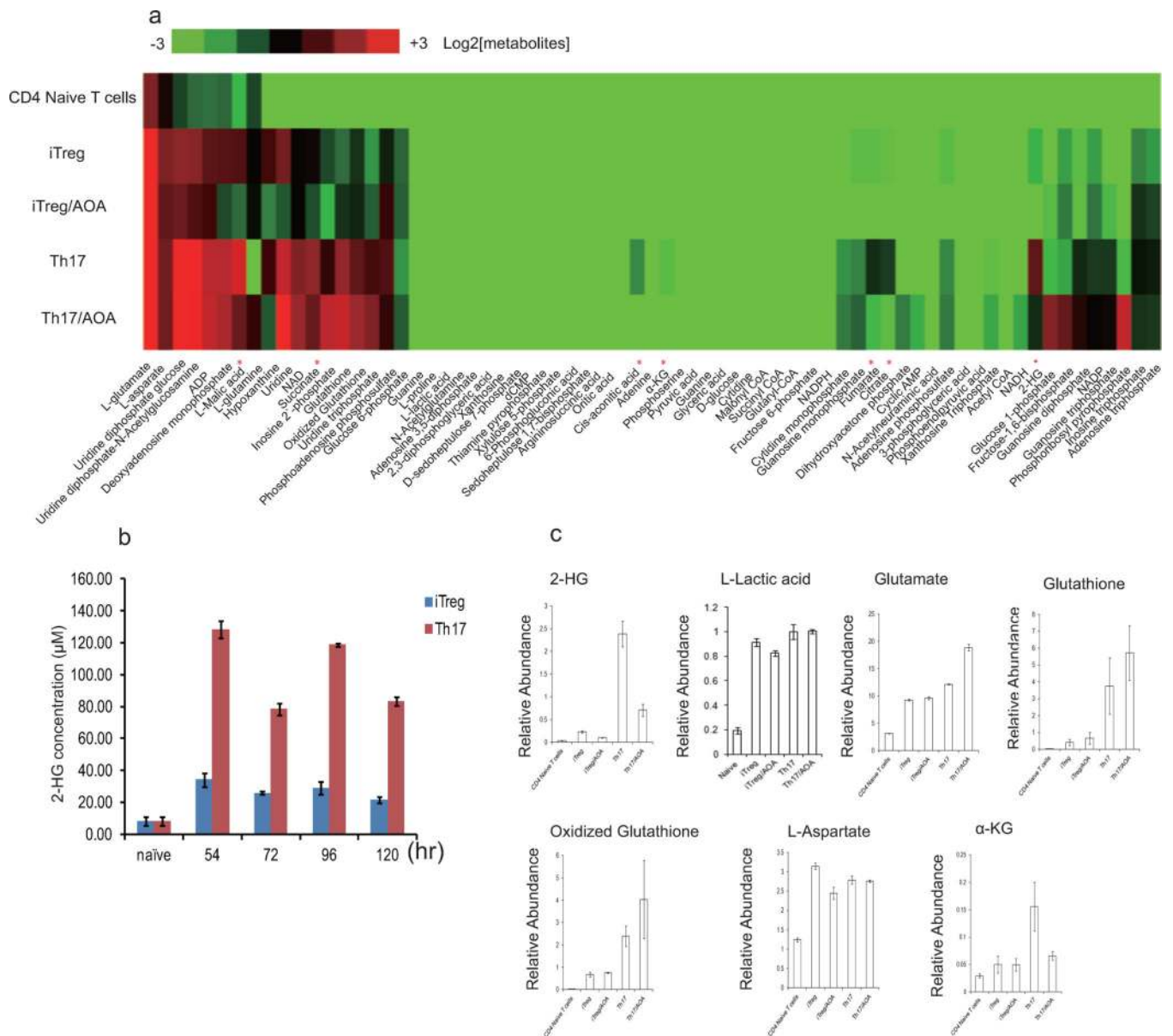
Extended Data Figure 3. Metabolic profiling of TH17 cells and iTreg cells. a) Intracellular metabolites profiling of differentiating TH17 cells and iTreg cells performed by LC/MS. * refer to the metabolites with differential abundance between TH17 cells and iTreg cell, which is inhibited by AOA. b) 2-HG concentration is much higher in differentiating TH17 cells than iTreg cells along differentiation time line. c) AOA significantly increased 2-HG, while does not affect the level of L-Lactic acid, glutathione, oxidized glutathione, L-aspartate, slightly decrease α-KG, slightly increase glutamate related to Extended Data Fig. 3a. The relative levels of 2-HG, L-lactic acid, L-glutamate, glutathione, oxidized glutathione, L-aspartate and α-KG from Extended Data Fig.3a were re-plotted in c. The data shown in b and c are mean±S.D. of three replicates from a representative experiment of three independent experiments.
