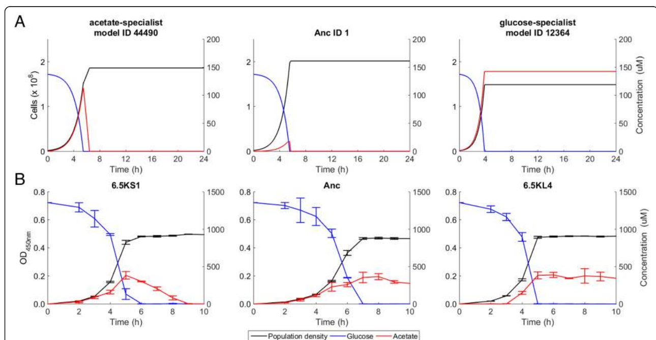
Fig. 3 Simulated and experimental dynamics of population density and substrate concentrations. a Simulated dynamics over a 24-h transfer cycle for the evolved acetate specialist (left, ID: 44490), ancestral (middle, ID: 1), and evolved glucose specialist (right, ID: 12364) model organisms. Model IDs are the same as in Fig. 1b. b Experimental data for the 6.5KS1 (left), ancestral (middle), and 6.5KL4 (right) clones from the LTEE. Biological experiments were performed at a 10-fold higher concentration of glucose than the simulations to increase cell density and thereby improve the accuracy of the measurements of cell growth and concentrations of residual glucose and secreted acetate. Biological data are means of three replicate cultures and error bars show standard deviations
