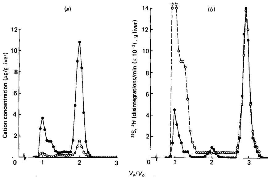
Fig. 1. Distribution of zinc and copper and the incorporation of radioactive amino acids into the liver cytosol of 5-d-old rats. (a) Distribution of Zn (●—●) and Cu (○---○); (b) distribution of ^{35}\text{S} (●—●) and ^3\text{H} (○---○). Animals were treated with 10 \mu\text{Ci} of both L-[ ^{35}\text{S} ]cysteine hydrochloride and L-[4,5- ^3\text{H} ]leucine and killed 4 h later. Liver cytosol was fractionated on Sephadex G75 (800 \times 15 mm) with Tris HCl buffer (10 mM, pH 8.0) as eluant.
