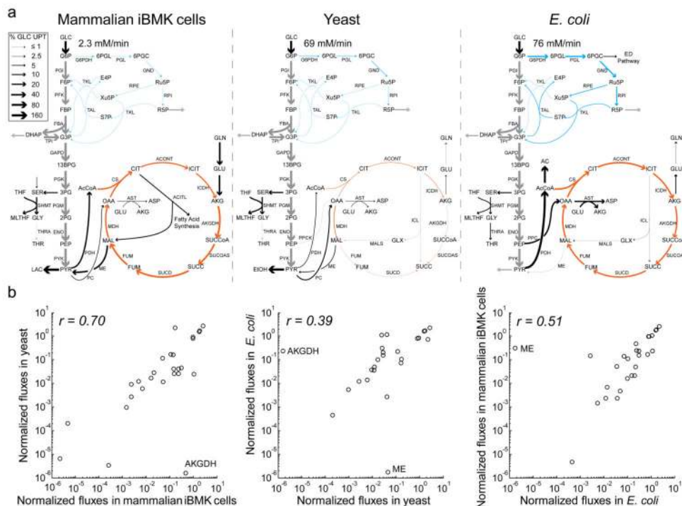
Figure 2. Metabolic flux distributions in mammalian iBMK cells, yeast, and E. coli
