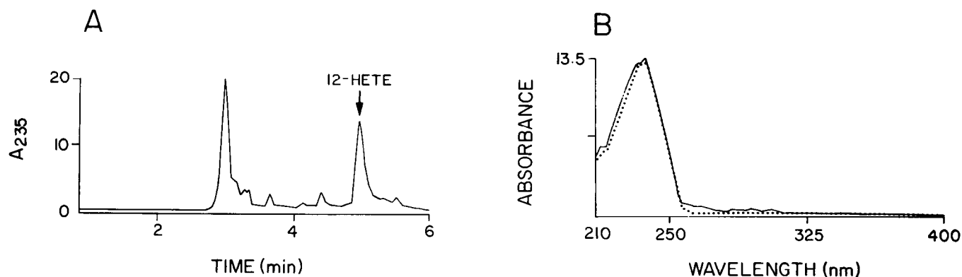
Figure 3. Identification of 12-HETE formed by Aplysia neural tissue analysis by UV spectrometry. The homogenate of neural ganglia from 100 animals was incubated with arachidonic acid ( 50 \mu\text{M} ) for 30 min, and the lipid extract was subjected to normal-phase HPLC purification (see Materials and Methods). A , A_{235} absorbance was monitored continuously. A major peak was observed at the retention time of the 12-HETE standard (4.8 min, indicated by the arrow). B , The full spectrum of this material (continuous line) was identical to that of authentic 12-HETE (dotted line).
