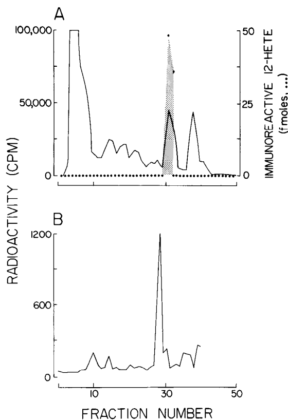
Figure 2. Identification of 12-HETE formed by Aplysia neural components. A , Reversed-phase HPLC and immunochromatography. Bath samples from neural components, incubated with ^3\text{H} -arachidonic acid (0.5 \mu\text{Ci} in 0.1 ml for 30 min), were subjected to reversed-phase HPLC (solvent system I); each 30 sec fraction was counted by liquid scintillation; the solid line (cpm) was drawn by connecting each point. The 2 major components that are separated from the solvent front eluted at the retention times of 12-HETE and 5-HETE. The material at the solvent front represents unidentified polar metabolites of arachidonic acid. The amounts of radioactivity on the chromatogram correspond to the production of the neural components from the cerebral, paired pleuropedal and abdominal ganglion of one specimen. In another experiment, bath samples from neural components incubated with arachidonic acid (15 \mu\text{M} ) were fractionated by HPLC and the material eluting at the retention time of 12-HETE was chromatographed again on the same HPLC system. After the second HPLC step, the eluted fractions were dried, reconstituted in phosphate buffer, and analyzed by radioimmunoassay, using commercial antibody against 12-HETE. The immunoreactive material, indicated by the shaded area, had the same retention time as did the 12-HETE standard. Recovery of standard ^3\text{H} -12-HETE after 2 chromatographic steps was typically 40–60% ( n = 3 ). B , Normal-phase HPLC. The radioactive material eluting with 12-HETE on reversed-phase HPLC was collected, dried, subjected to methylation, and chromatographed by normal-phase HPLC. The major radioactive component was eluted at the retention time of 12-HETE methyl ester. Recovery was only 10–20%.
