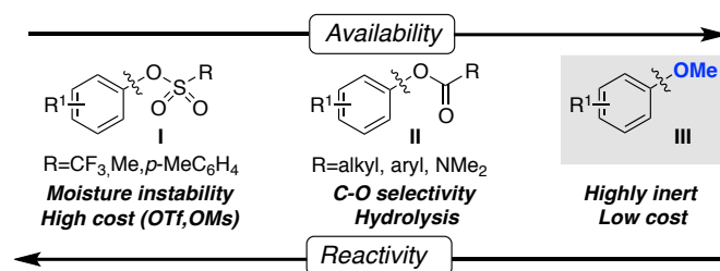
Scheme 1. C–O electrophiles in metal-catalyzed cross-coupling reactions.
