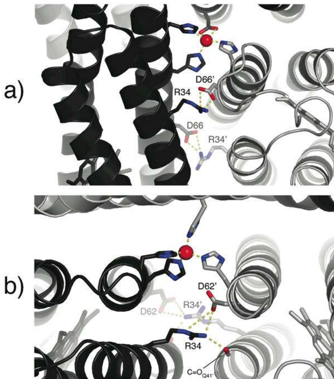
Figure 3. Interfacial H-bonding interactions in Zn 4 :MBPC-1 4 (a) and Zn 4 :MBPC-2 4 (b) assemblies that involve R34 and D66 in the former and R34 and D62 in the latter. The pairwise interactions shown above are repeated twice due to the internal twofold symmetry of each tetrameric assembly.
