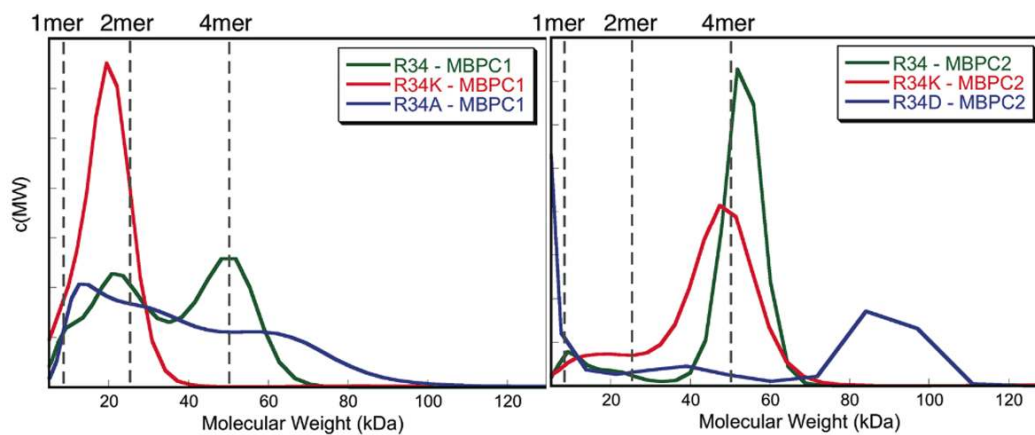
Figure 4. Molecular weight distributions of MBPC-1 (left) and MBPC-2 (right) species as determined by sedimentation velocity measurements. All samples contain 600 \mu\text{M} protein and 600 \mu\text{M} Zn, with the exception of R34A-MBPC-1, which contains 300 \mu\text{M} Zn. 13
