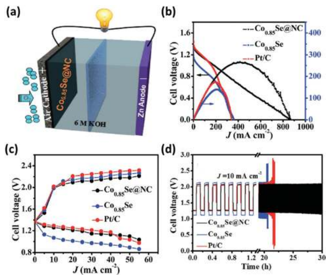
Fig. 14 Electrochemical performance of the \text{Co}_{0.85}\text{Se}@NC cathode incorporated Zn-air battery: (a) Schematic representation of rechargeable Zn-air battery. (b) Polarization plot ( V-i ) and associated power density plot. (c) Charge/discharge potential ( V-i ) plots. (d) Cyclic stability performance. Reprinted with permission. 25 Copyright 2017 Royal Society of Chemistry.
