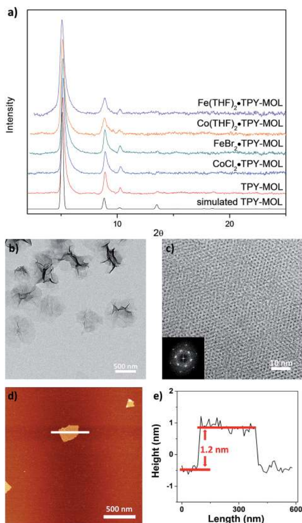
Fig. 2 (a) PXRD patterns of TPY-MOL, CoCl_2 ·TPY-MOL, FeBr_2 ·TPY-MOL, Co(THF)_2 ·TPY-MOL, and Fe(THF)_2 ·TPY-MOL in comparison to simulated PXRD pattern for TPY-MOL; (b) TEM image of TPY-MOL; (c) HRTEM image and fast Fourier transform (FFT) pattern of TPY-MOL; (d) tapping-mode atomic-force microscope (AFM) topographic image of TPY-MOL; (e) height profile along the white line of TPY-MOL.
