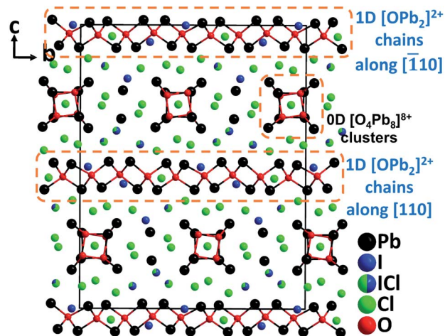
Fig. 13 Crystal structure of \text{Pb}_{18}\text{O}_8\text{Cl}_{15}\text{I}_5 viewed along the a -axis (Pb–Cl and Pb–I bonds have been omitted for clarity).
