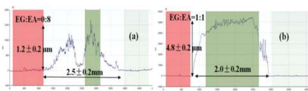
Fig. 4 Surface profiles of a silver ink film after sintering: (a) coffee ring effect; (b) a flat film without the coffee ring using suitable solvent composition. Reproduced with permission from ref. 46. Copyright 2012, Royal Society of Chemistry.
