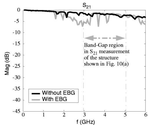
Fig. 20. Measured S_{21} of the structures shown in Fig. 15.
