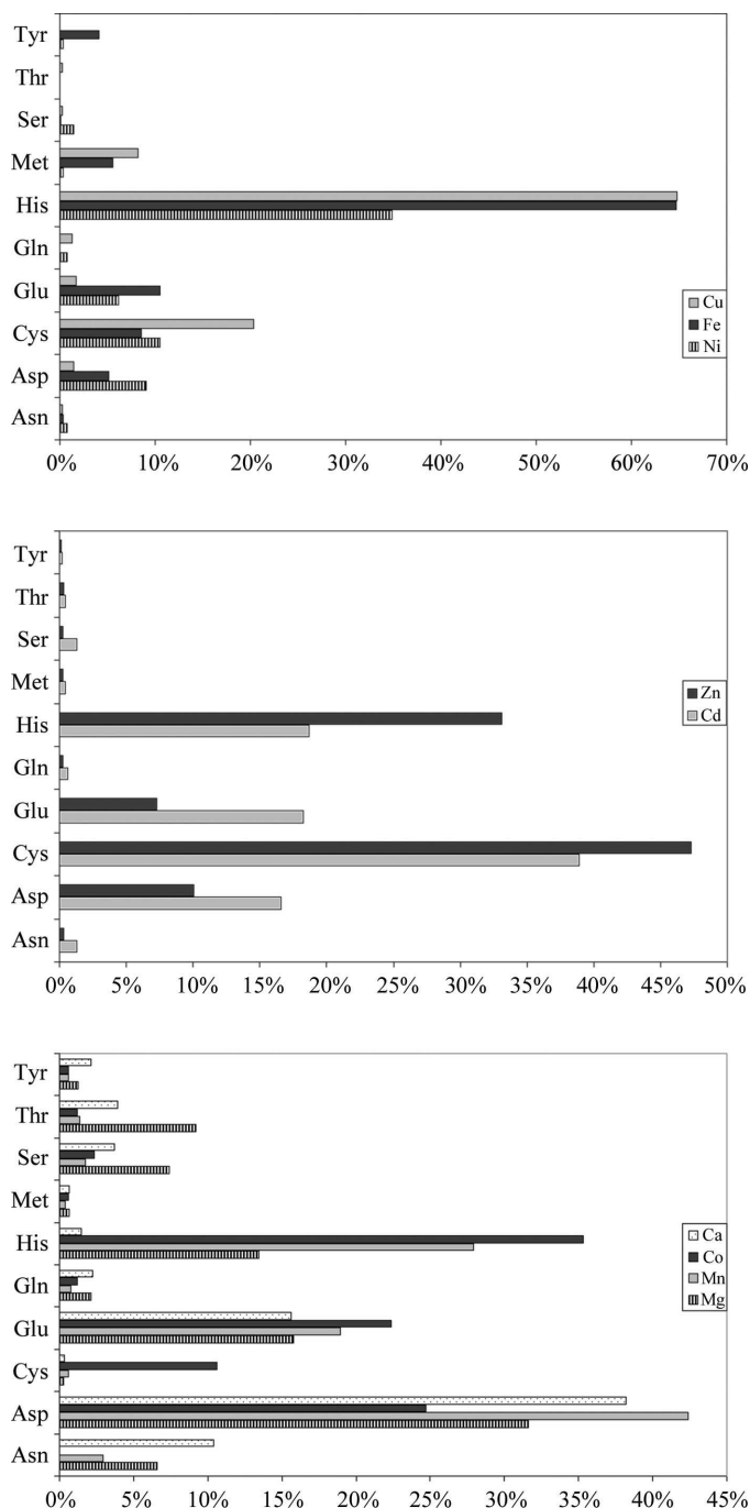
Figure 2 Percentage of metal sites in which the amino-acid side-chain functional group is present as an electron-donating group. Statistics are only given for the amino-acid residues that most often participate in metal coordination (Asn, Asp, Cys, Gln, Glu, His, Met, Ser, Thr and Tyr). The metal ions are grouped according to the similarity of their coordination spheres: Cu 2+ , Fe 2+ and Ni 2+ (top), Zn 2+ and Cd 2+ (middle) and Ca 2+ , Mn 2+ , Mg 2+ and Co 2+ (bottom).
