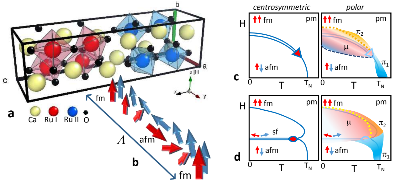
FIG. 4: Crystal structure of \text{Ca}_3\text{Ru}_2\text{O}_7 , panel a shows the Ru atoms occupy a single crystallographic site. The antiferromagnetic primary order splits these positions into two double layers, Ru (I) and Ru (II), which have internally ferromagnetic spin-configurations and are antiparallel. Above 48 K transition the collinear spin-structure has moments directed along the a -axis of the orthorhombic cell. The polar axis is b . Cartesian coordinates xyz are used for spin and spatial gradients, with z along b as indicated. Panel b shows a metamagnetic one-dimensional texture propagating along the a axis. In an applied field along the polar axis b , the spin configuration oscillates from fm to afm and back to fm over a repeat period \Lambda . c, d , schematic phase diagrams of bipartite antiferromagnets with easy-axis anisotropy. Panel c the temperature-field phase diagram for the case of large anisotropy. A first-order transition between an antiferromagnetic (afm) collinear and a spin polarized (fm) state occurs along the double line. For temperatures above a tricritical point (triangle) the transition is continuous. The afm-fm co-existence can be replaced in a polar magnet by a region of modulated phases \mu . Towards the paramagnetic state at elevated temperatures, anomalous transitions into precursor states ( \pi_1, \pi_2 ) then are expected. The dotted yellow line indicates the transition between the improper, metamagnetic texture and the precursor state \mu \rightarrow \pi_2 . The precursor of type \pi_1 only implies modulations of primary afm modes, while \pi_2 states can be metamagnetic, being composed of modulations between afm and fm modes. Panel d displays the phase diagram of a system with a weak anisotropy. The double line signifies a first order transition of the spin-flop type, which is only a re-orientation of the ordered moment. The marked point is a bi-critical point (almond mark). In an antiferromagnet with a polar structure, metamagnetic textures \mu can still occur at elevated temperatures and for fields higher than the spin-flop field, when a sizeable net moment and antiferromagnetic order compete. As in the case of large anisotropy, different types of precursors, i.e. a proper antiferromagnetic texture \pi_1 or metamagnetic textures with coupled modulations between afm and fm mode \pi_2 can occur.
