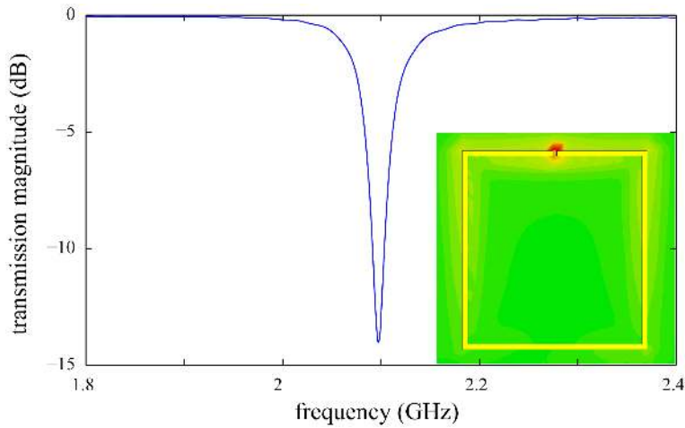
Figure 2. Numerically resolved transmission magnitude of the SRR-loaded microstrip. (Inset) Absolute electric field strength over the surface of the structure at 2.1 GHz. The results are for the structure in Fig. 1(a), and are determined with a commercial full-wave electromagnetic solver, CST Microwave Studio, based on the Finite-Integration Technique (FIT).
