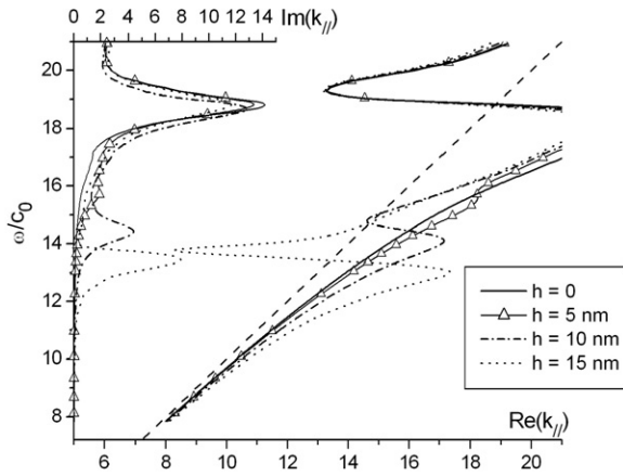
Figure 5. Dispersion relations of the pole of the scattering matrix representing the surface plasmon constant of propagation ( k_{||} = k_p ) for the grating given in figure 1(a) with d = 60 nm, c/d = 1/7 , and different groove depths as indicated in the figure. The lower axis and curves on the right are for the real parts of the pole, the upper axis and curves on the left are for the imaginary parts of the pole. All units in \mu\text{m}^{-1} . The dashed line is the light cone.
