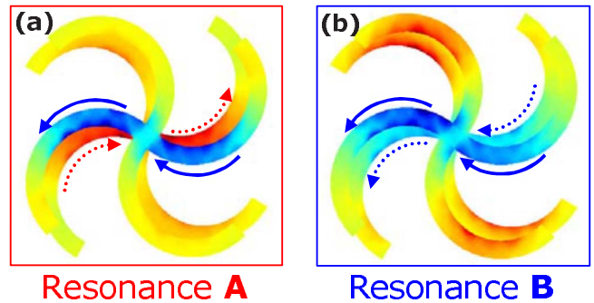
FIG. 4. (Color online) Current modes leading to a negative refractive index. The antisymmetric current mode (a) is excited by RCP at 4.7 GHz and the symmetric current mode (b) is excited by LCP at 6.2 GHz. The horizontal component of the excited currents is shown, where blue and red correspond to currents in opposite directions.
