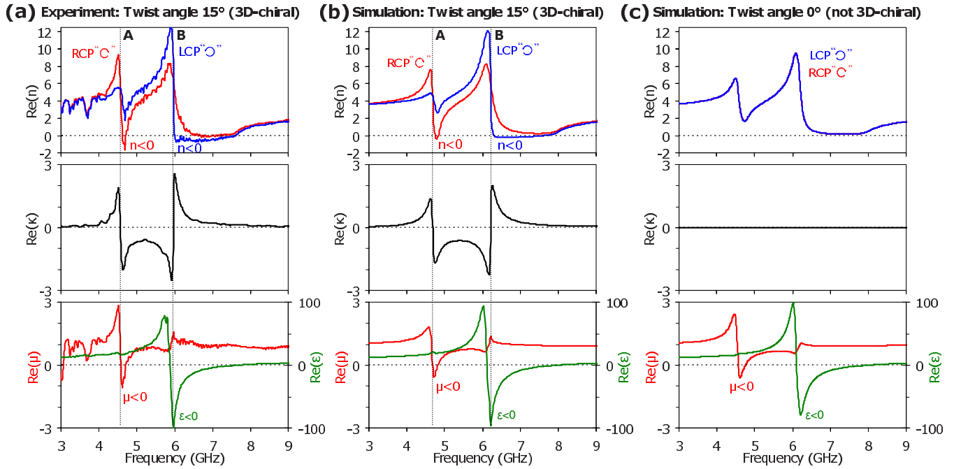
FIG. 3. (Color online) Effective medium parameters of the bilayered metamaterial. Experimental (a) and numerical (b) results for refractive index n (top), chirality parameter \kappa (middle), and permeability \mu and permittivity \epsilon (bottom) are shown for the 3D-chiral bilayered metamaterial. (c) Effective parameters derived from numerical simulations for a bilayered metamaterial with no relative twist between layers of rosettes. Note that \epsilon and \mu are almost identical for both cases. Negative n in the 3D-chiral case arises from the contribution of the large chirality parameter \kappa .
