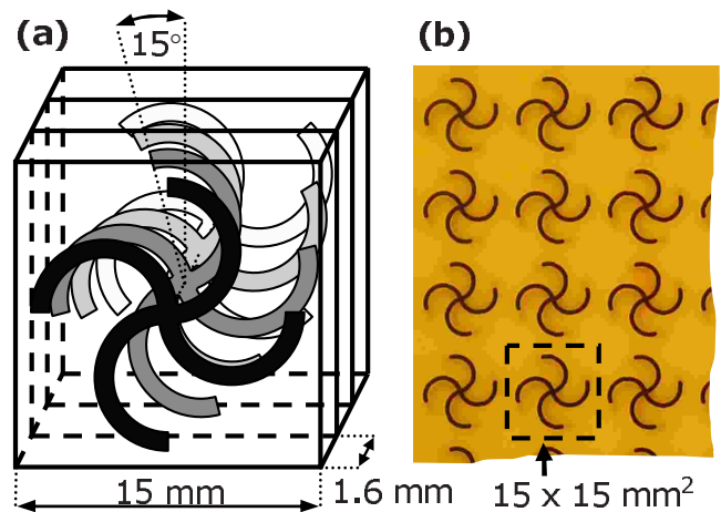
FIG. 1. (Color online) Structure of the metamaterial. (a) Schematics of the four-layered metamaterial's unit cell. The rosettes in neighboring layers have a relative twist of 15^\circ . The structure of metamaterials with a different number of layers is analogous. (b) Photograph of part of a bilayered metamaterial sheet. The twisted rosettes of the second layer can be seen as a shaded area thanks to partial transparency of the substrate. A unit cell has been marked.
