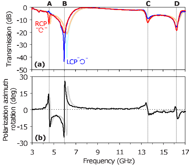
FIG. 2. (Color online) Circular dichroism and optical activity of the bilayered metamaterial. Measurements (dark lines) and numerical simulations (faint lines) are shown. (a) Transmission levels for left-handed (blue, LCP, - ) and right-handed (red, RCP, + ) circularly polarized waves. (b) Azimuth rotation for linearly polarized waves.
