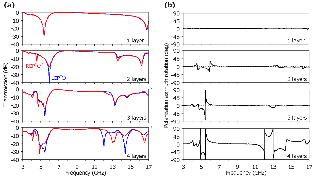
FIG. 6. (Color online) Development of the metamaterials' transmission characteristics when increasing the number of layers from one to four. (a) Transmission spectra measured for the metamaterials' circular eigenpolarizations LCP (blue, - ) and RCP (red, + ). (b) Polarization azimuth rotation measured for linear polarization.
