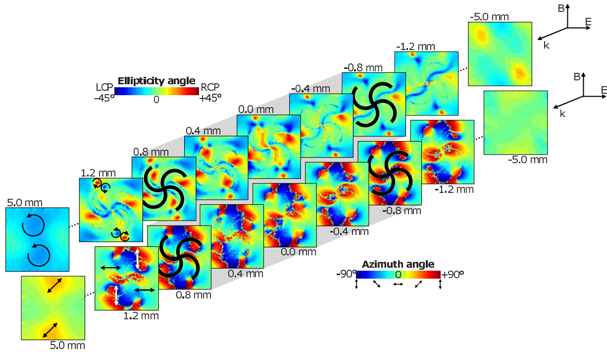
FIG. 5. (Color online) Polarization state evolution for the total field as a linearly polarized wave propagates through the bilayered metamaterial at 4.6 GHz. The top sequence shows the ellipticity angle of the total field, while the bottom sequence shows the polarization azimuth.
