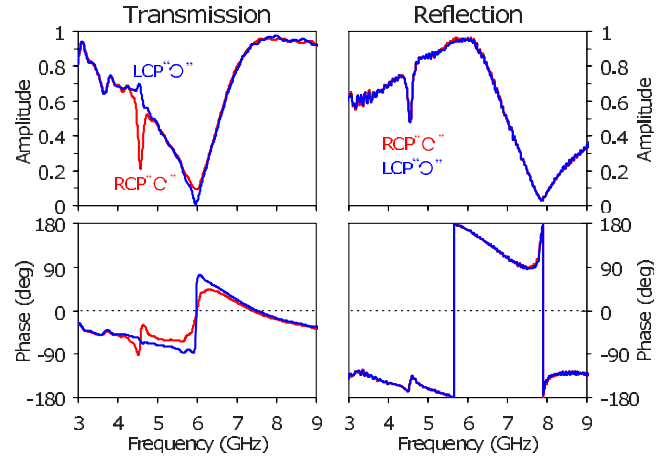
FIG. 7. (Color online) Amplitude and phase of the complex transmission and reflection coefficients T and R measured for the 3D-chiral bilayered metamaterial.
