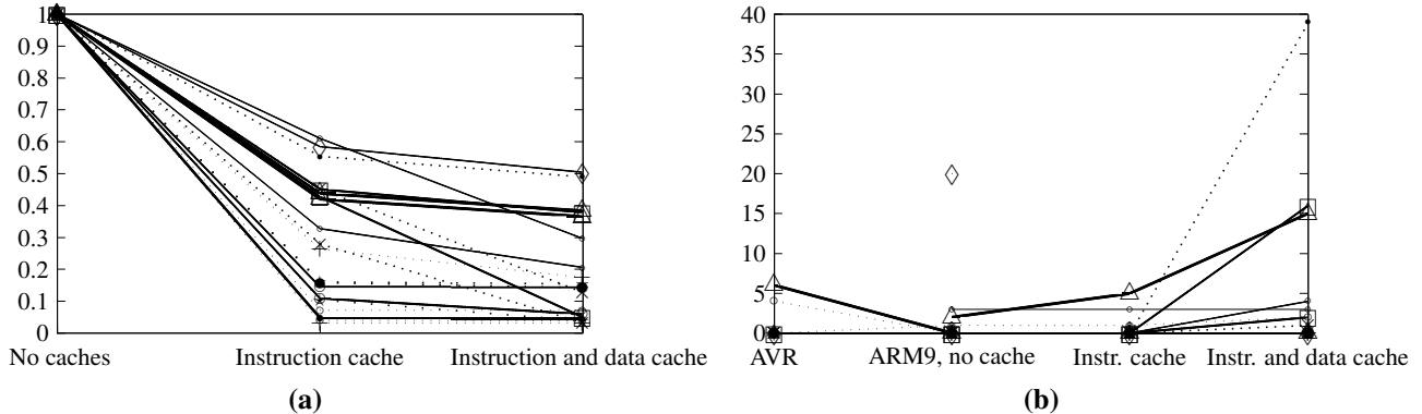
Figure 6. (a) Improvement in WCET estimate by precisely modelling the different caches on the ARM9. The average improvement in WCET estimate is 71.6% by modelling the instruction cache, and 81.3% by modelling both caches. (b) Analysis times for the different configurations in minutes. The average successful analysis times are, respectively: 52.46 secs., 83.61 secs., 44.8 secs. and 265.75 secs.
