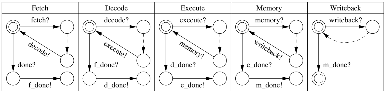
Figure 3. Sketch of the UPPAAL model for the pipeline in the ARM9TDMI processor core.
