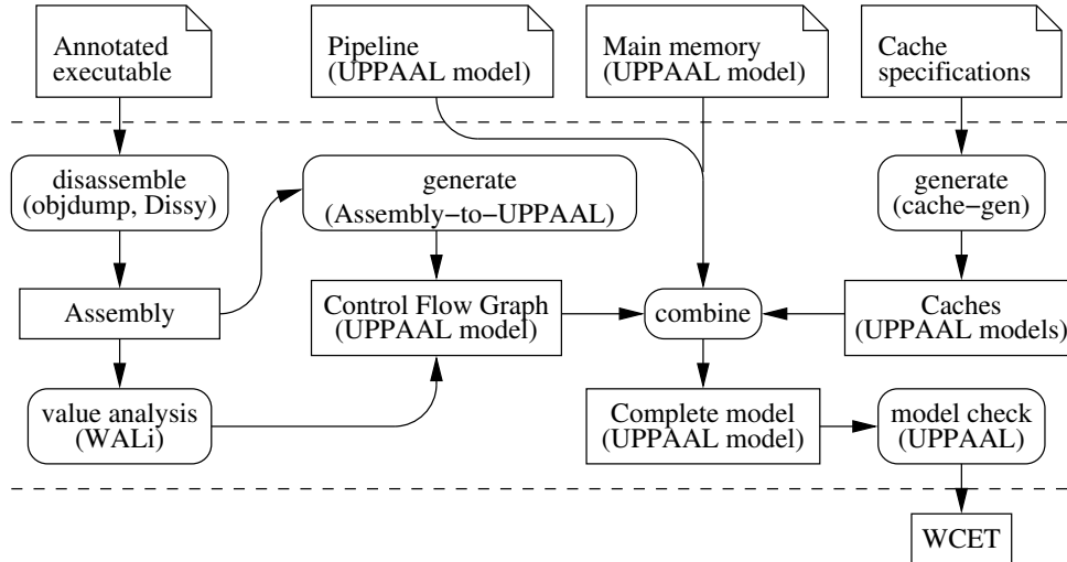
Figure 1. Overview of the prototype implementation of METAMOC. The top row shows required inputs. The executable (annotated with loop bounds) is the only user input, whereas the other inputs are platform specific models developed by specialists or hardware vendors. The output is a WCET estimate for running the executable on the hardware platform. Rounded and rectangular boxes represent actions and objects, respectively.
