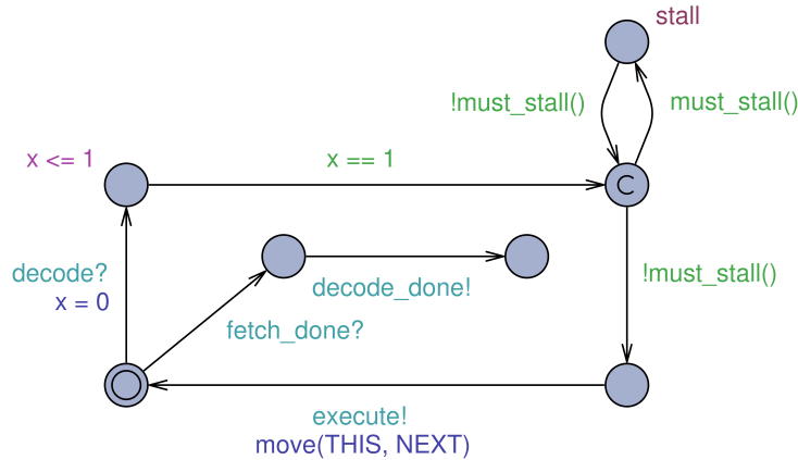
Figure 4. UPPAAL model for the decode stage in the ARM9TDMI pipeline, with x being a local clock.
