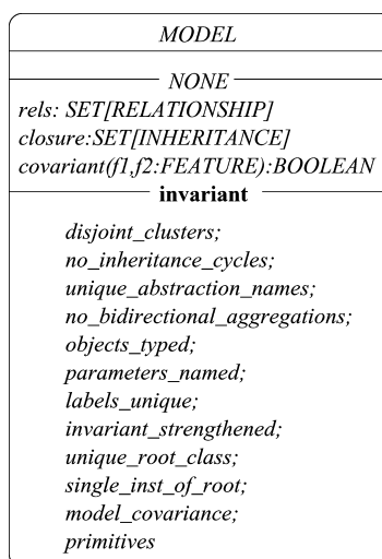
Fig. 6. Interface of class MODEL .
