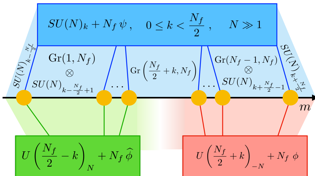
Figure 10. Phases of large- N QCD 3 (shown in blue) with 0 \leq k < \frac{N_f}{2} as a function of the flavor-singlet mass m . There are N_f + 1 phases, which generically contain both NG bosons (with Grassmannian target spaces) associated with different patterns of flavor-symmetry breaking, as well as a Chern-Simons TQFT in the deep IR. There are N_f first-order phase transitions indicated by yellow dots. The same phases and transitions are captured by the two mutually non-local bosonic dual theories (shown in green and red), if their respective scalar potentials are chosen appropriately.
