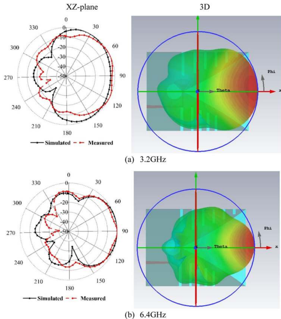
Figure 8. Simulated and measured radiation pattern at (a) 3.2 GHz and (b) 6.4 GHz.
