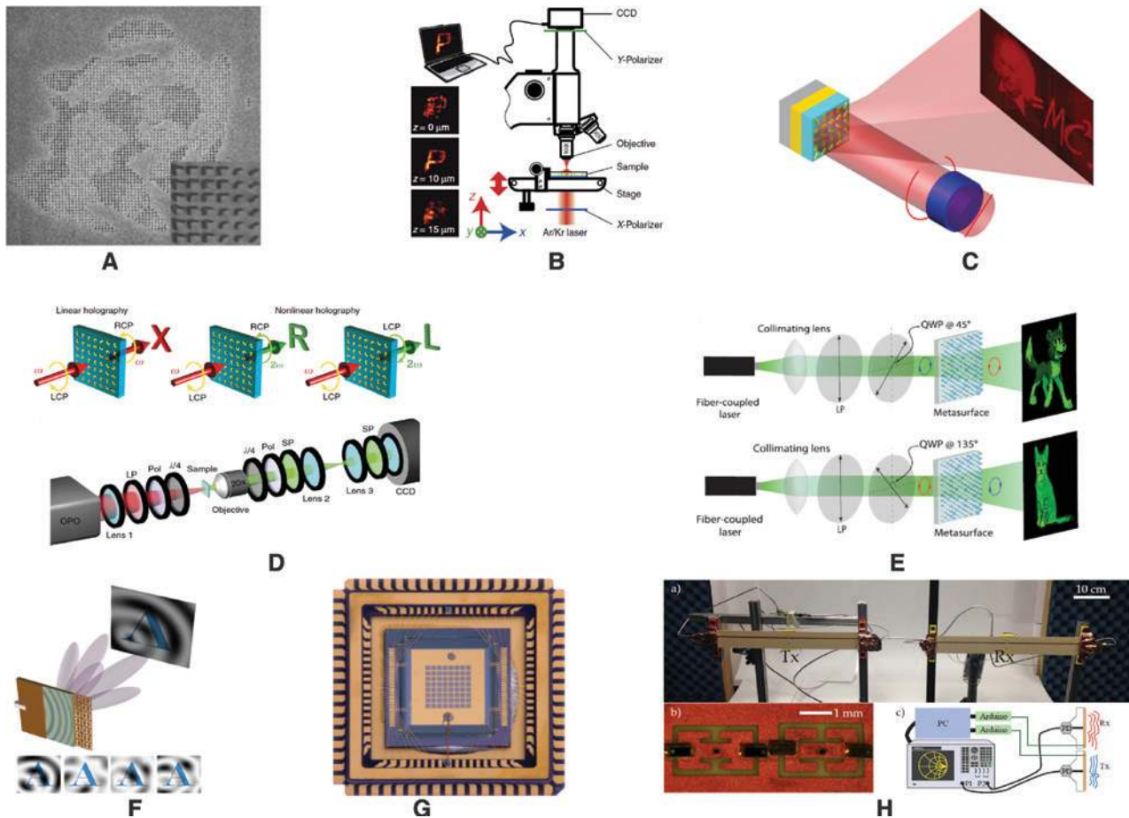
Figure 12: Metasurface applications at optical and microwave frequencies.
