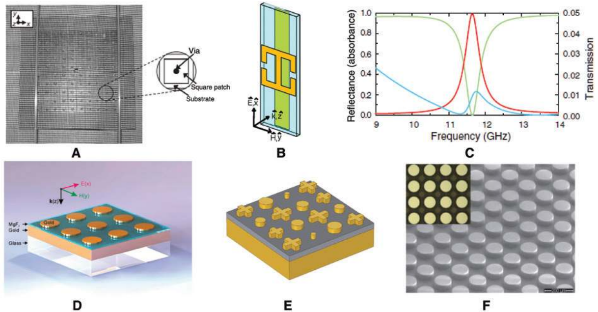
Figure 4: Passive metasurface absorbers from microwave to optical frequencies. (A) Resistive sheet topped high impedance surface as a microwave absorber. (B) Unit cell of perfect metamaterial absorber. (C) Absorption simulation results of surfaces in (A). (D) Infrared perfect absorber. (E) Broadband solar absorber. (F) THz all-dielectric metasurface absorber.
