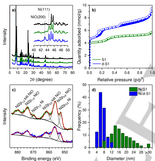
Figure 1. a) XRD analysis of parent S1 (black), Ni/S1 (green) and Ni/d-S1 (blue). b) N_2 physisorption analysis performed at 77K. c) XPS analysis of the Ni 2p_{1/2} and 2p_{3/2} level. d) Ni particle size distribution based on 200 TEM measurements.
