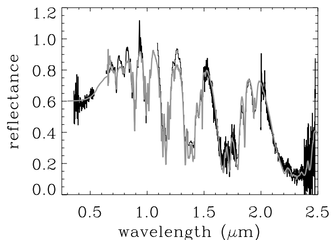
FIG. 7.—Complete spectral fit for 2005 FY9. The model uses 1\ \text{cm} methane grains intimately mixed with 10\ \mu\text{m} grains of tholin and 100\ \mu\text{m} ethane grains in a 60:30:10 mix. All features of the spectrum are fitted, except for slight mismatches in the infrared continuum level. The continuum mismatches are well within the range of variation of the infrared reflectance of the many different possible tholin-type materials that might be present on the surface.
