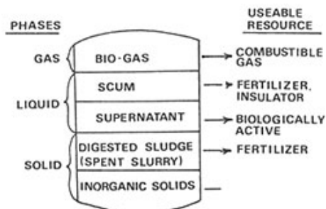
FIG.2 Layering of By-Products In the Digester
