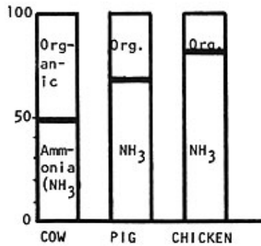
FIG.12 Types of Nitrogen Found in Different Kinds of Manure
