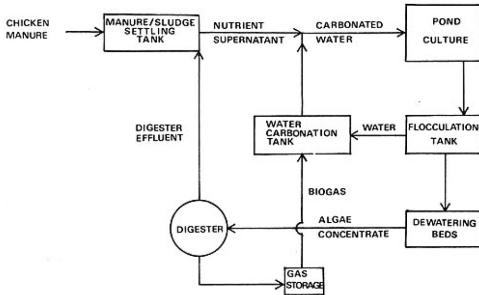
FIG.17 Flow Diagram of Sludge-Algae-Methane Conversion System
