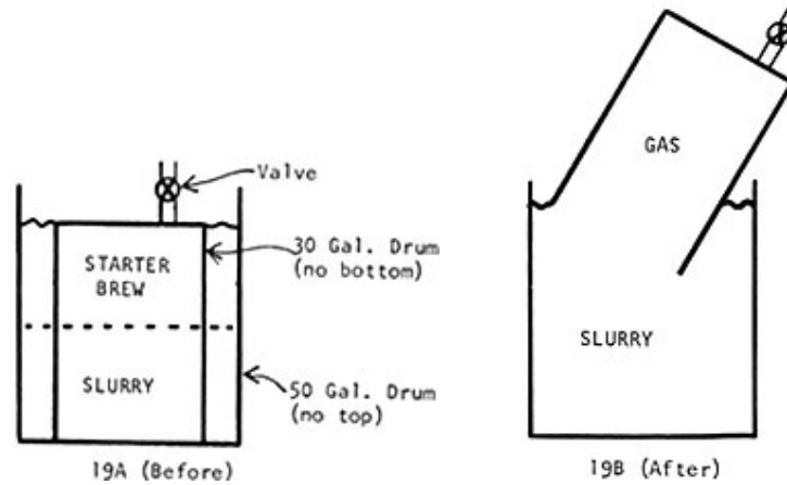
Fig. 19A & B: Sump digester before and after methane Production
