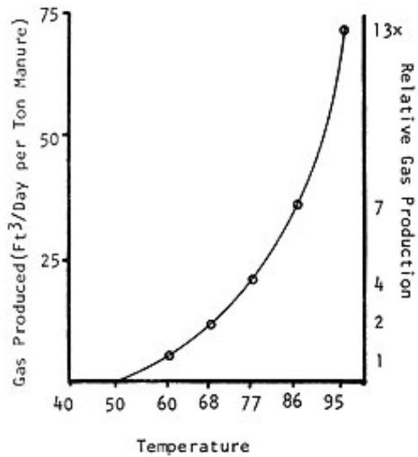
FIG.9 Gas Production and Temperature (after Ref. 15)
