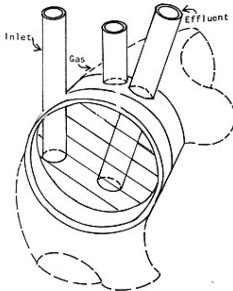
FIG.24 Placement of Pipes In Plastic Cylinder (Note Angle of Pipes)
