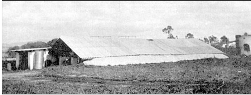
Engine room, summer cooling tank and digester on the first full scale methane power plant to operate on the linear displacement principle. Water heating tower on right was abandoned in the first year.
