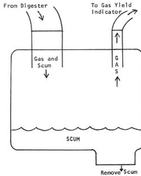
Fig. 27 Scum collector
