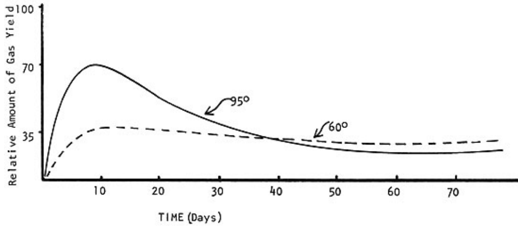
FIG.10 Comparison of Gas Production Rates at 60°F and 95°F (Measured from time new sludge added to buffered digester).
