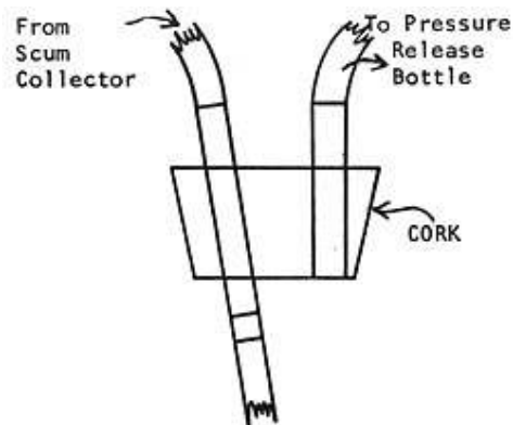
FIG.28 Gas Yield Indicator
