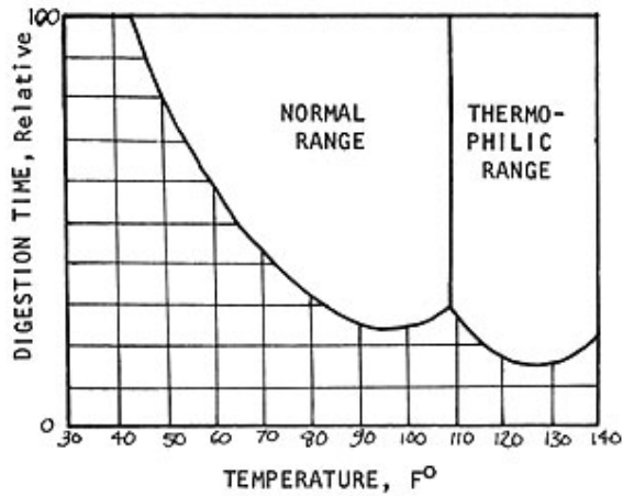
FIG.8 Digestion Time and Temperature (after Ref. 7)
