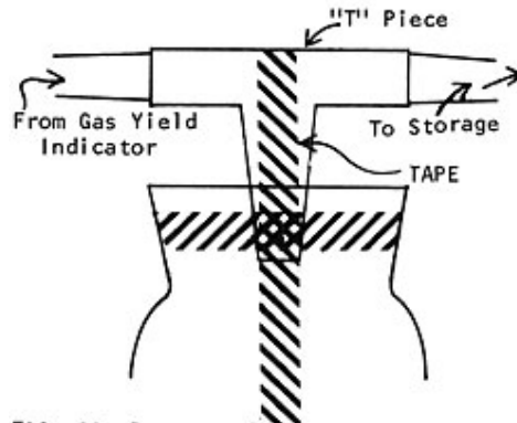
FIG. 29 Pressure Release
