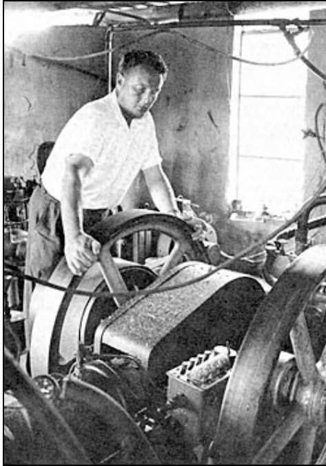
Fig. 34 13 hp diesel engine converted to run on methane gas
