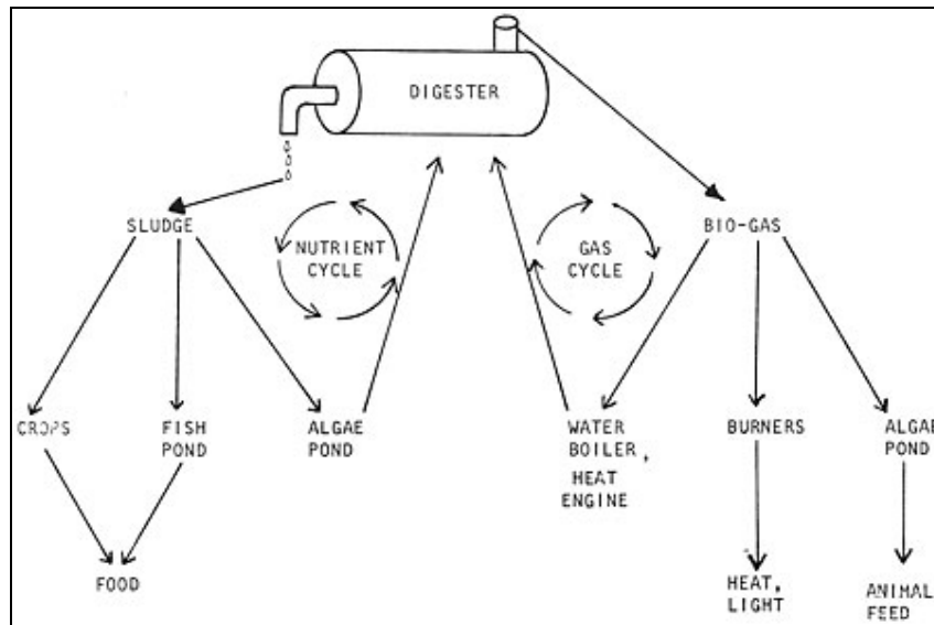
Fig. 4 The closed nutrient system of a complete digester operation
