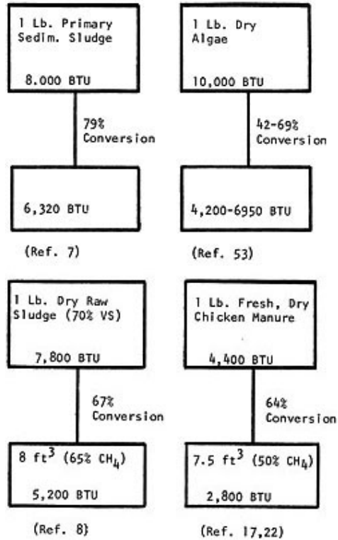
FIG.15 Efficiency of Methane Production from Different Materials
