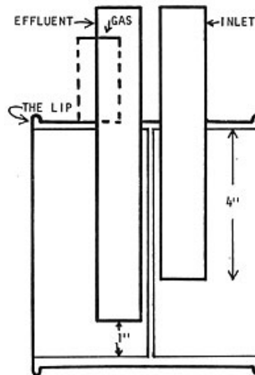
Fig. 23 Cross section of the plastic insert
