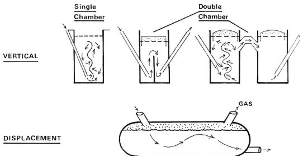
FIG.13 Types of Continuous-Feeding Digesters
