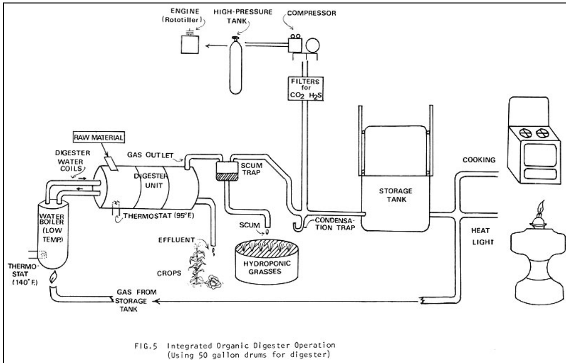
Fig. 5 Integrated organic digester operation (using 50 gallon drums for digester)
