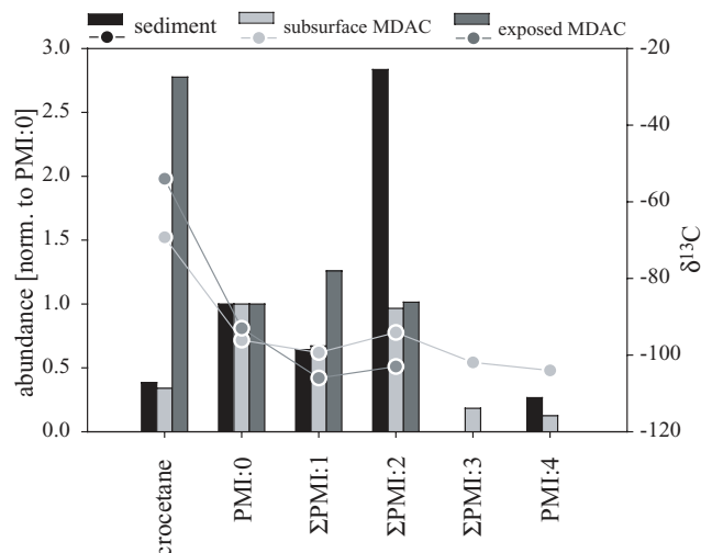
Fig. 8. Abundance (bars) and stable carbon isotope composition (circles) of archaeal, isoprenoid hydrocarbon lipids extracted from sediments and MDACs of the AOM zone (155 cm b.s.f.) of core 1904 and from surface MDACs recovered by a ROV. Abundances were normalised to PMI:0. Note that concentrations of crocetane are ca. 7.5-fold increased in surface MDACs. Low concentrations prohibited \delta^{13}\text{C} -measurements of hydrocarbons in the sediment.
