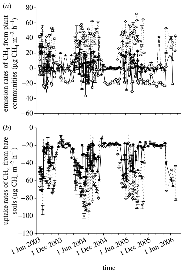
Figure 2. (a) Methane emission rates from different plant communities (squares, shrub community in a Potentilla meadow; circles, grass community in a Kobresia meadow; filled up-triangles, grass community in a Potentilla meadow) and (b) methane uptake rates from bare soils (open down-triangles, bare soils in a Kobresia meadow; filled circles, bare soils in a Potentilla meadow) over the 3 years' observation period. Mean \pm s.e. of three replicates are presented.
