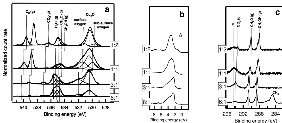
Figure 2: (a) O1s photoelectron spectra of a copper sample at 400 °C in CH 3 OH:O 2 reactant streams of 1:2, 1:1, 3:1, and 6:1. Raw data are shown as dots, the result of the fits as solid black lines. The incident photon energy was 720 eV. Gas phase peaks are found at BEs > 534 eV, the surface peaks are at BE < 534 eV. In CH 3 OH:O 2 =1:2 and 1:1 the Cu 2 O peak dominates the surface XPS spectrum. The Cu 2 O peak is absent in the spectra that were taken under reducing conditions (CH 3 OH:O 2 =3:1, 6:1). In those spectra the sub-surface oxygen peak is the strongest peak in the surface part of the spectrum. (b) Corresponding valence band spectra. The spectrum taken in oxidizing conditions (CH 3 OH:O 2 =1:2) shows a typical shape for a Cu 2 O sample with a gap \Delta at 0.9 eV BE, thus confirming the observation from the O1s spectrum in (a). The spectrum taken in CH 3 OH:O 2 =1:1 shows that the surface consists of a mixture of metallic copper and Cu 2 O. The spectra measured under reducing conditions (CH 3 OH:O 2 =3:1, 6:1) exhibit the typical valence band spectrum for metallic Cu, which confirms the absence of a Cu 2 O peak in the O1s spectra in (a). (c) C1s spectra taken under the same conditions as in (a) and (b). CO 2 , CH 3 OH and CH 2 O gas phase peaks are observed. There are no carbon-containing species at the surface, only for CH 3 OH:O 2 =6:1 a peak is visible at 284.7 eV, probably due to decomposition products of methanol that accumulate at the surface. The peak at 294.3 eV is due to some potassium contamination.
