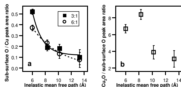
Figure 4: (a) Sub-surface O-to-Cu stoichiometry under reducing conditions as a function of the inelastic mean free path of the photoelectrons. The concentration of sub-surface oxygen close to the sample surface is higher for the oxygen-rich atmosphere ( CH_3OH:O_2=3:1 ). Deeper into the sample the concentration of sub-surface oxygen is similar for the two different atmospheres. (b) Sub-surface oxygen-to- Cu_2O peak area ratio as a function of the inelastic mean free path of the photoelectrons under oxidizing conditions ( CH_3OH:O_2=1:2 ). Cu_2O is predominantly located at the sample surface.
