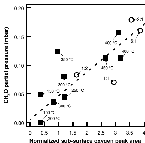
Figure 5: Partial pressure of formaldehyde as a function of the sub-surface oxygen peak area for the spectra in Fig. 1a (open circles), and for a different experiment (black squares) in which the temperature was varied in the range from 150 °C to 450 °C at a constant \text{CH}_3\text{OH}:\text{O}_2 mixing ratio of 3:1 (the same total pressure as for the spectra in Fig. 1a). The partial pressure of formaldehyde is linearly correlated to the abundance of sub-surface oxygen in the near-surface region. The dashed line is a linear fit of the data points.
