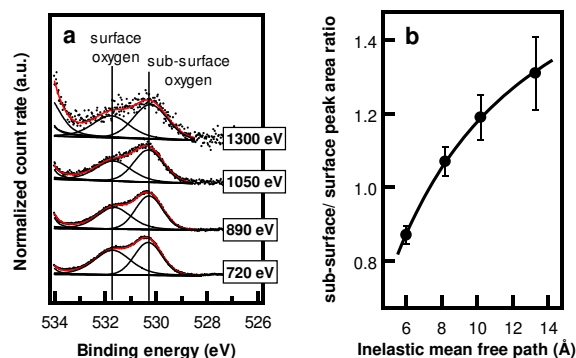
Figure 3: (a) O1s spectra as a function of incident photon energy in CH_3OH:O_2=3:1 at 400^\circ C . The incident photon energy is indicated for each spectrum. In the fits of the peaks their relative BE position was kept constant, as well as the ratio of their FWHM. The FWHM ratio was kept constant instead of the absolute values to account for the decrease of the spectral resolution with increasing incident photon energy, which leads to a broadening of the peaks. (b) Peak area ratio of the sub-surface oxygen (530.4 eV) and surface oxygen (532.0 eV) O1s peaks calculated from the peak areas in (a). The relative increase of the spectral weight of the 530.4 eV peak with increasing inelastic mean free path indicates that this species is located below the 532.0 eV species, in the sub-surface region. The spacing between neighboring atomic layers in Cu in the [100] direction is 1.8 \text{ \AA} . The solid line is a least squares fit of the data points using I_{530.4}/I_{532.0}=n_{530.4}/n_{532.0}\exp[-(z_{532.0}-z_{530.4})/\lambda] , with I as integrated intensity of the peak, n the concentration in atom percent, z the average depth below the surface, and \lambda the inelastic mean free path. The fit parameters are n_{530.4}/n_{532.0}=1.8 , and z_{532.0}-z_{530.4}=4 \text{ \AA} .
