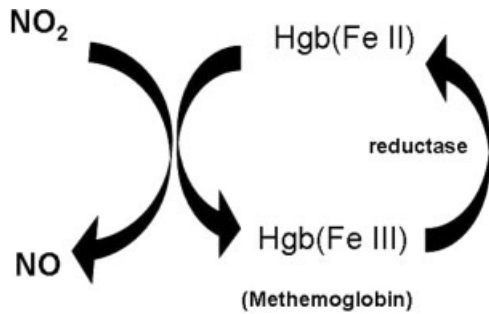
Fig. 5. Hemoglobin acts as a nitrite reductase, but only in the deoxygenated form. This is a reduction in contrast to the reaction of \text{NO}_2 with oxygenated hemoglobin ( \text{HgbFe(II)(O}_2 ), which is an oxidation.
