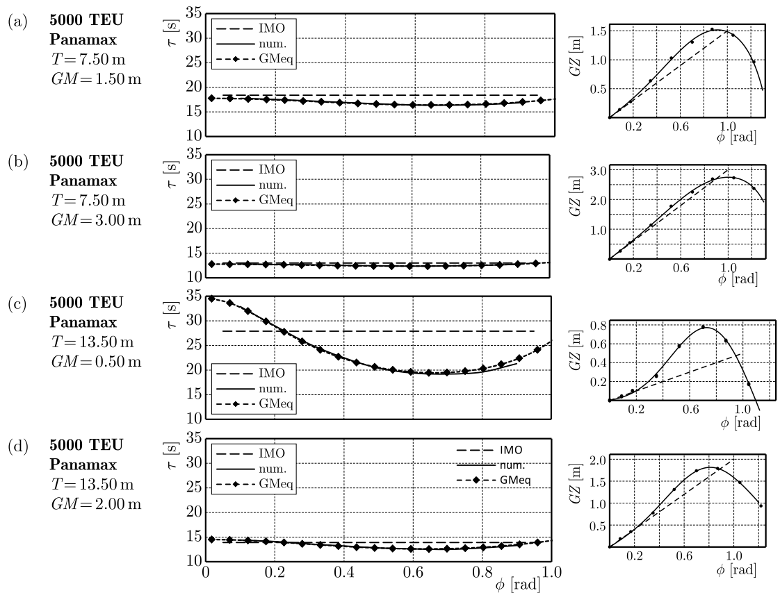
Fig. 5. Rolling period vs. rolling amplitude for the 5000 TEU Panamax container ship (left plot) and the corresponding GZ curve and the metacentric triangle (right plot)
