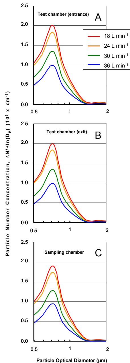
Fig. 3. The particle size distributions of aerosolized B. atrophaeus endospores measured at three different points of the experimental system and at four different air flow rates.
