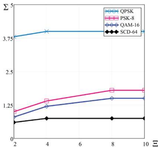
Fig. 6. Results of modeling the influence of the number of paths on the maximum permissible inter-symbol interference value for the equally probable pulse response of the channel
