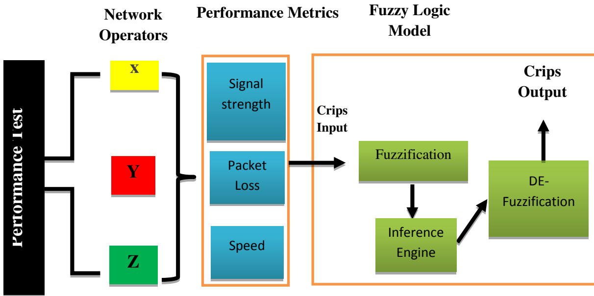
Fig 1: Architecture of the Proposed Model
