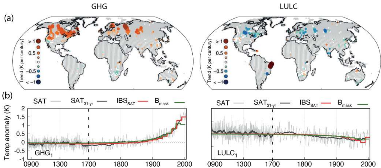
Figure 7. (a) Spatial distribution of linear trends in SAT – GST anomalies over the 1850–2005 CE period evaluated at every grid point collocated with a borehole site in the GHG- and LULC-only ensemble mean (left and right in a, respectively). Only grid points delivering statistically significant trends ( p < 0.05 ) are colored. (b) LM global SAT annual anomalies and the corresponding 31-year filtered outputs and the global IBS_{SAT} and the B_{mask} pseudo-reconstructions for the GHG_1 and LULC_1 ensemble members. Note the different discretization in the x axis after 1700 CE.
