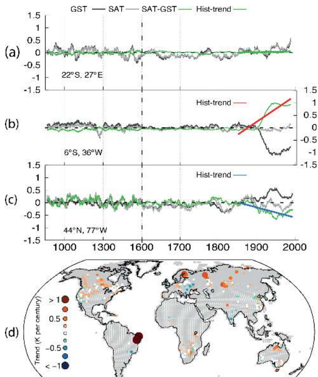
Figure 5. LM evolution of SAT and GST anomalies, SAT minus GST, and the linear trends of SAT minus GST over the 1850–2005 CE period for three different grid points with borehole records in ALL- F_2 as an example. Each grid point illustrates a possible case of the long-term SAT–GST relationship: (a) strong coupling during the LM, (b) decreasing GST relative to SAT and (c) increasing GST relative to SAT during industrial times. (d) Spatial distribution of linear trends in SAT minus GST anomalies over the 1850–2005 CE period evaluated at every grid point with the presence of a borehole site using the ALL- F ensemble mean. Grid points showing statistically significant trends ( p < 0.05 ) are colored in red/blue depending on whether they are increasing/decreasing SAT–GST trends.
