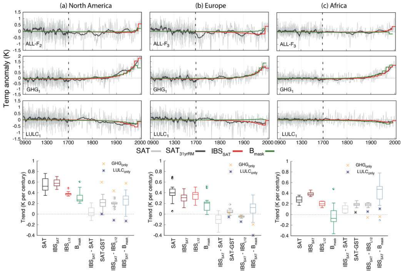
Figure 8. LM regional SAT annual anomalies and the corresponding 31-year filtered outputs and the global IBS_{SAT} and the B_{mask} pseudo-reconstructions for the ALL-F_2 , GHG_1 and LULC_1 (from top to bottom) members of the ALL-F , GHG - and LULC -only ensembles, respectively, (a) North America, (b) Europe and (c) Africa. Note the different discretization in the x axis after 1700 CE. Bottom panels as Fig. 6b but for each of the regions presented.
