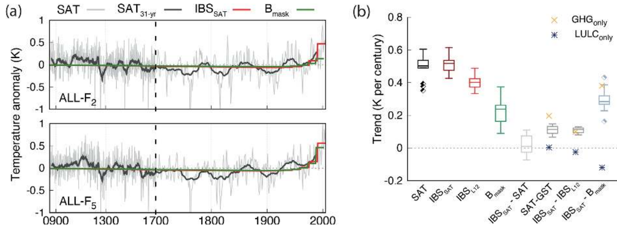
Figure 6. (a) LM global SAT annual anomalies and the corresponding 31-year filtered outputs and the global IBS SAT and B_{\text{mask}} pseudo-reconstructions for the ALL- F_2 and ALL- F_5 members of the ALL- F ensemble. Note the different discretization in the x axis after 1700 CE. (b) Estimated linear fit as Fig. 2b, but the SAT, IBS SAT , IBS L12 , B_{\text{mask}} and the differences between IBS SAT - SAT, SAT - GST, IBS SAT - IBS L12 and IBS SAT - B_{\text{mask}} cases are represented. Additionally, the ensemble medians of the GHG- and LULC-only ensembles are indicated by the crosses and asterisks, respectively, in the IBS SAT - IBS L12 and the IBS SAT - B_{\text{mask}} columns.
