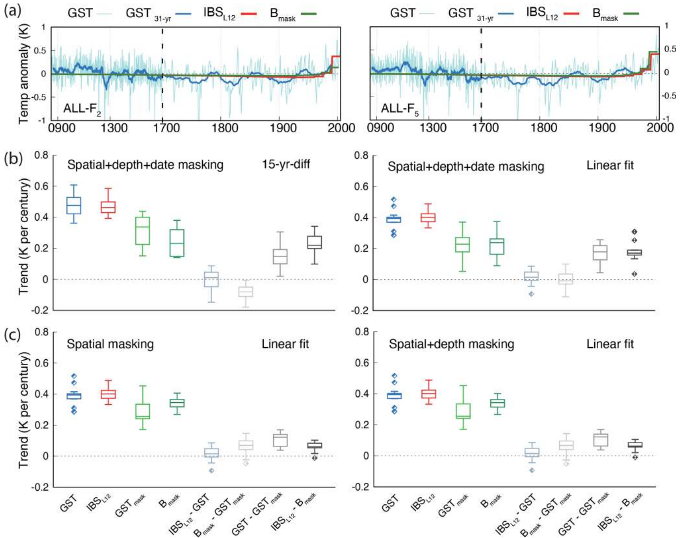
Figure 2. (a) LM global GST annual anomalies and the corresponding 31-year filtered output and the global IBS L12 and B mask pseudo-reconstructions for the ALL-F 2 and ALL-F 5 members of the ALL-F ensemble. Note the different discretization in the x axis after 1700 CE. (b) Boxplots describing the centennial trends over the period 1900–2005 CE, calculated for each of the 13 ensemble members within ALL-F after applying space, depth and time masking in the model to mimic real BTP distribution. Boxplots of trend differences have been created by subtracting individual trends, following Santer et al. (2008). Panel (c) as in (b) but applying spatial and depth masking (right) and only spatial masking (left). GST, IBS L12 , GST mask , B mask and the differences between IBS L12 – GST, B mask – GST mask , GST – GST mask and IBS L12 – B mask cases are represented. Trends are presented as the 15-year-difference case (b left; see text) and the linear fit to the data calculated over an annual basis (b right). The 25th, 50th and 75th percentiles are indicated, and the whiskers represent the lowest/highest value within 1.5 interquartile range (IQR) of the 25th/75th percentile. Outliers are indicated as diamonds in the same color of the box. They represent the values lower/higher than the lower/upper whisker. Note that colors in (a) correspond with those in (b) and (c).
