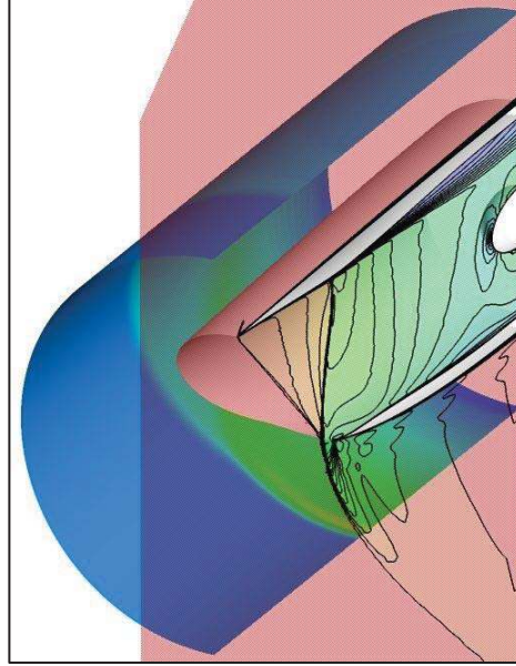
Figure 17. Sound pressure contours on a cylinder about a STEX-Circular inlet.
