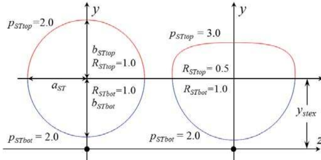
Figure 3. Two examples of tracing curves defined using super-ellipses.
