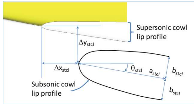
Figure 7. Defining the profile of the subsonic cowl lip.
