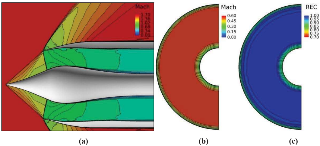
Figure 13. Images of the flowfield for the axisymmetric spike inlet: (a) Mach number contours on the symmetry plane, (b) Mach number contours at the engine face, and (c) total pressure recovery contours at the engine face.
