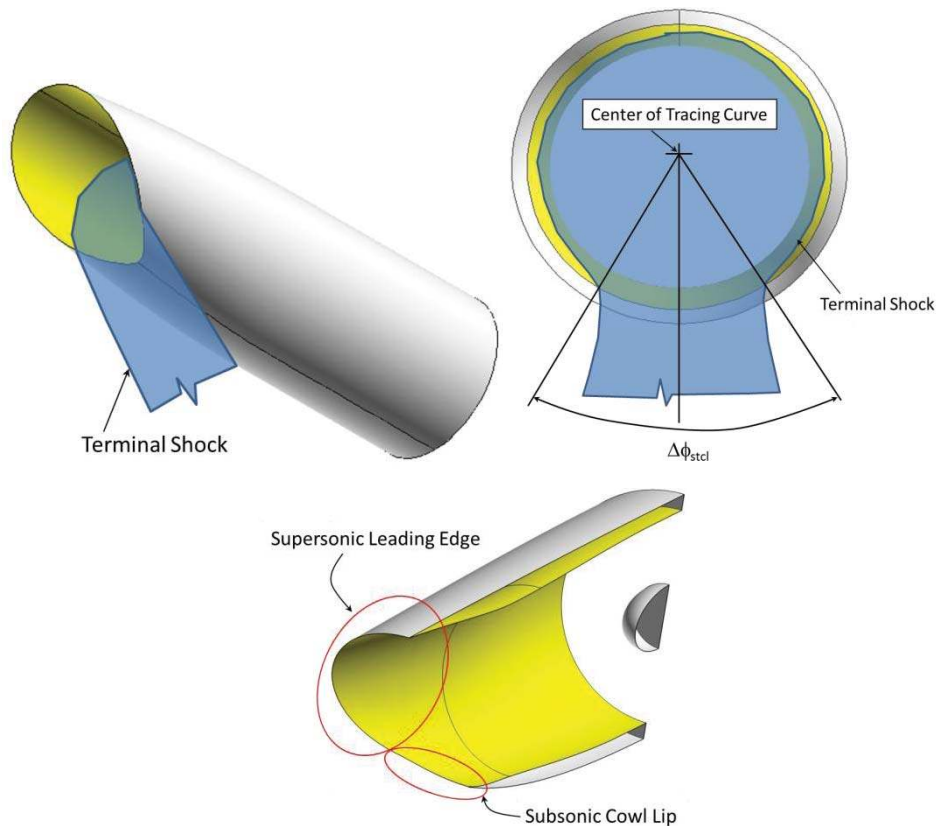
Figure 6. The supersonic leading edge and the subsonic cowl lip.
