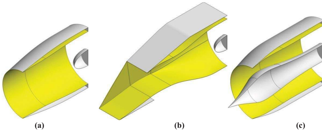
Figure 10. Images of the three traditional inlets designed by SUPIN: (a) axisymmetric pitot inlet, (b) two-dimensional inlet, and (c) axisymmetric spike inlet.
