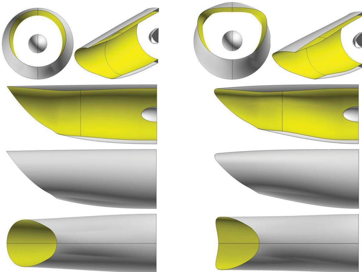
Figure 5. Examples of streamline-traced inlets with the tracing curves of Fig. 3.
