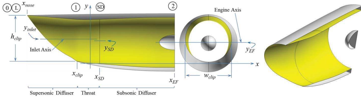
Figure 1. Schematic of a streamline-traced external-compression
