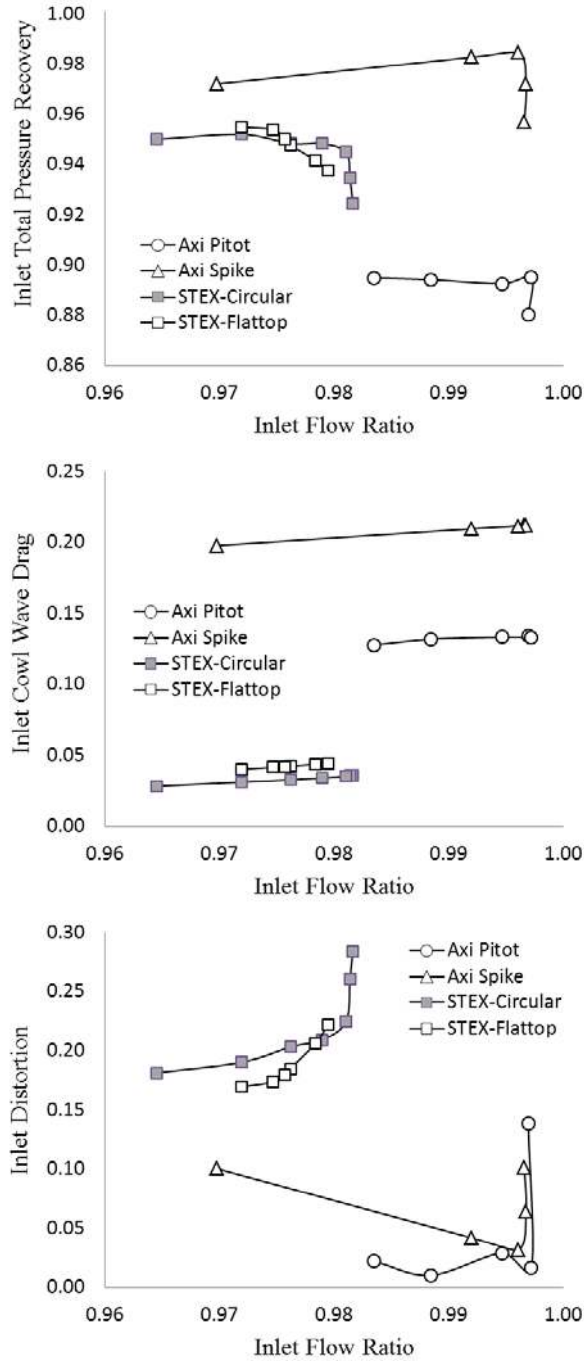
Figure 11. Characteristic performance curves from the CFD simulations of the inlets.
