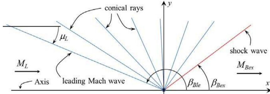
Figure 2. Axisymmetric Busemann flow field.
