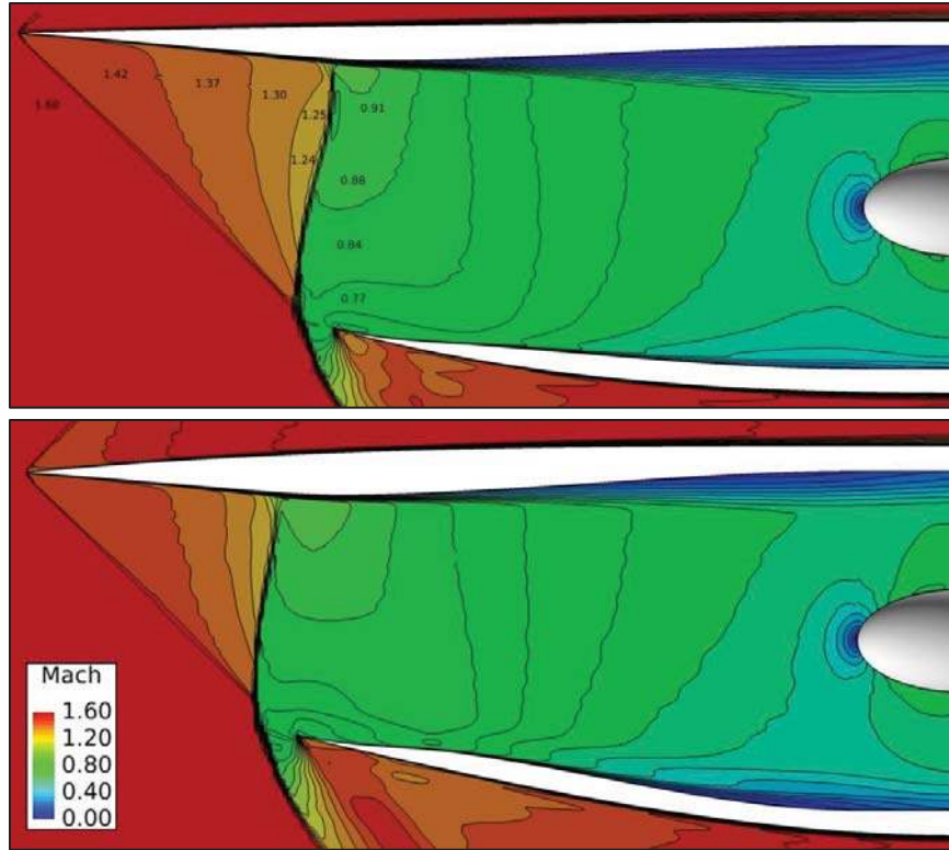
Figure 14. Mach number contours on the symmetry plane for the STEX-Circular (top) and STEX-Flattop (bottom) inlets.
