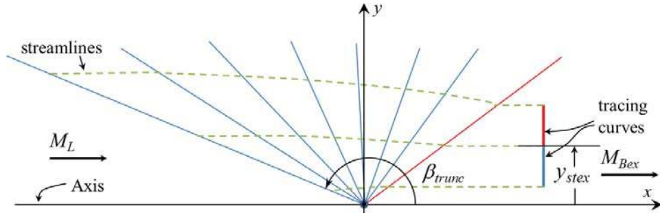
Figure 4. Integration of streamlines from the tracing curve.
