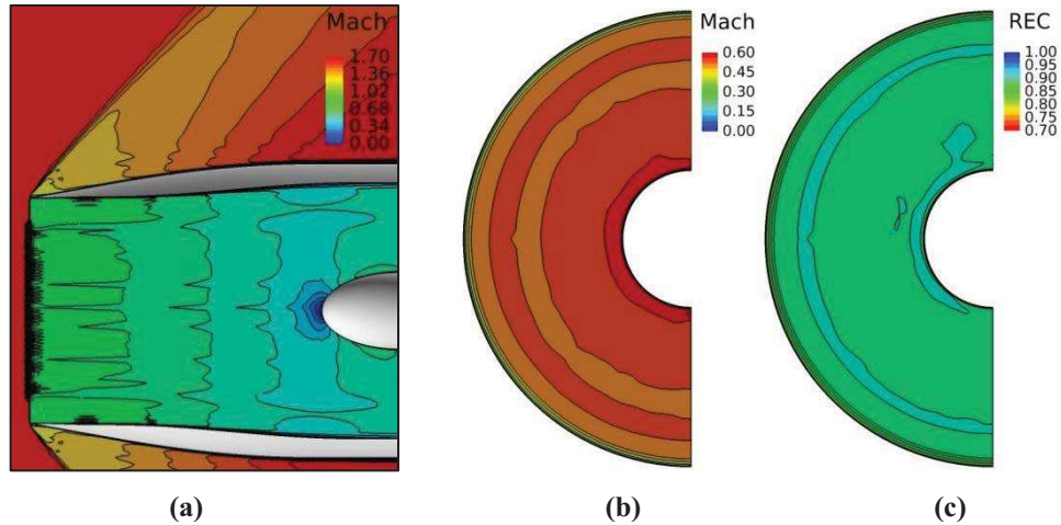
Figure 12. Images of the flowfield for the axisymmetric pitot inlet: (a) Mach number contours on the symmetry plane, (b) Mach number contours at the engine face, and (c) total pressure recovery contours at the engine face.
