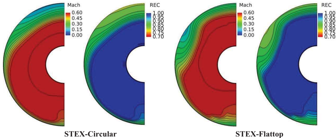
Figure 16. Mach number and total pressure recovery contours at the engine face of the STEX-Circular (left) and STEX-Flattop (right) inlets.
