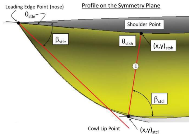
Figure 8. Cowl lip and shoulder modifications.
