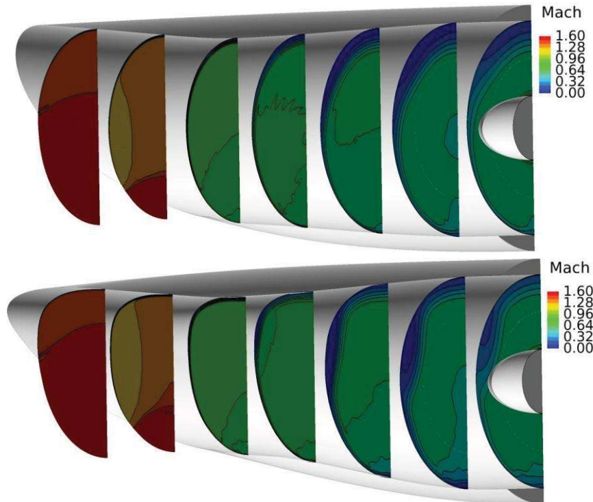
Figure 15. Mach number contours at axial stations for the STEX-Circular (top) and STEX-Flattop (bottom) inlets.
