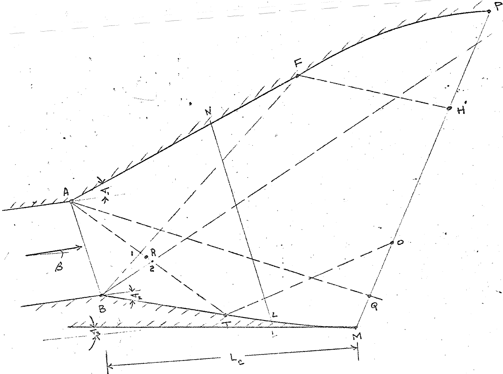
FIGURE 5. WAVE DIAGRAM
