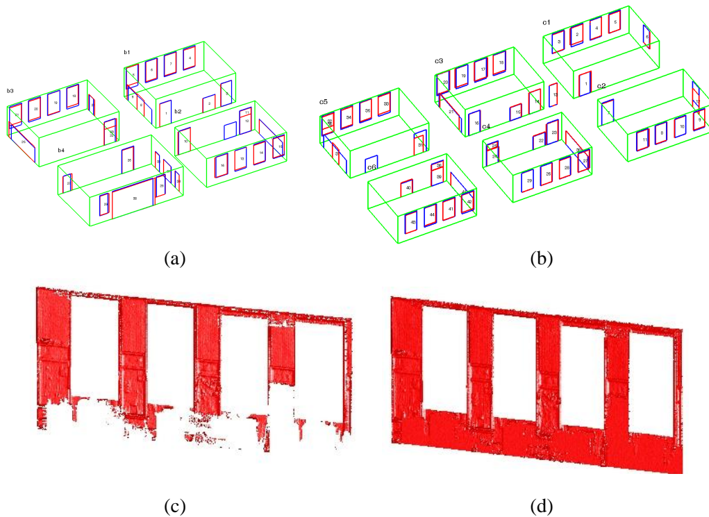
Figure 7. Detailed planar surface modeling results. (a-b) Reconstructed model of the facility corresponding to the first floor (a) and second floor rooms (b). The detected openings are shown in red, while the ground truth openings are shown in blue. (c-d) Occlusion region reconstruction shown before (c) and after (d) occluded regions have been filled in.
