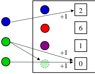
Fig. 3 Counter based data structure: the blue (top) item is already stored, so its count is incremented when it is seen. The green (middle) item takes up an unused counter, then a second occurrence increments the counter by one.
