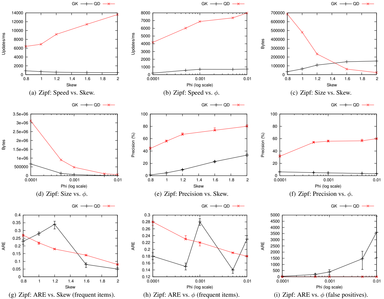
Fig. 9 Performance of quantile algorithms on synthetic data
