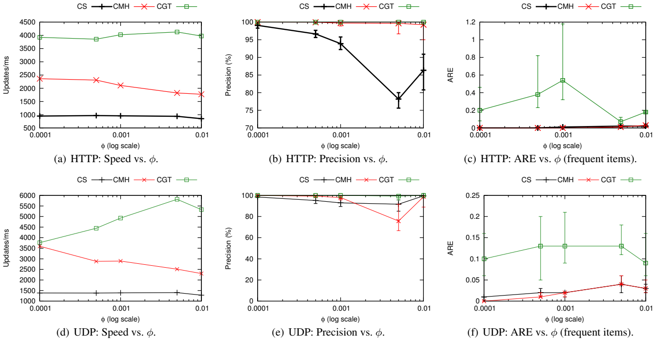
Fig. 14 Performance of sketch algorithms on real network data
