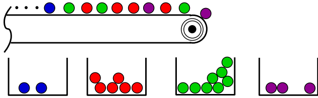
Fig. 1 A stream of items defines a frequency distribution over items. In this example, with a threshold of \phi = 20\% over the 19 items grouped in bins, the problem is to find all items with frequency at least 3.8 — in this case, the green and red items (middle two bins).
