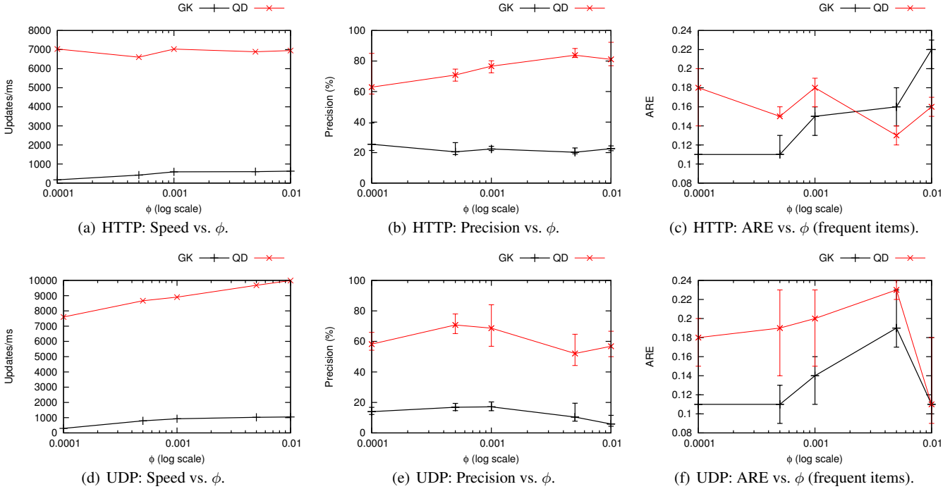
Fig. 10 Performance of quantile algorithms on real network data
