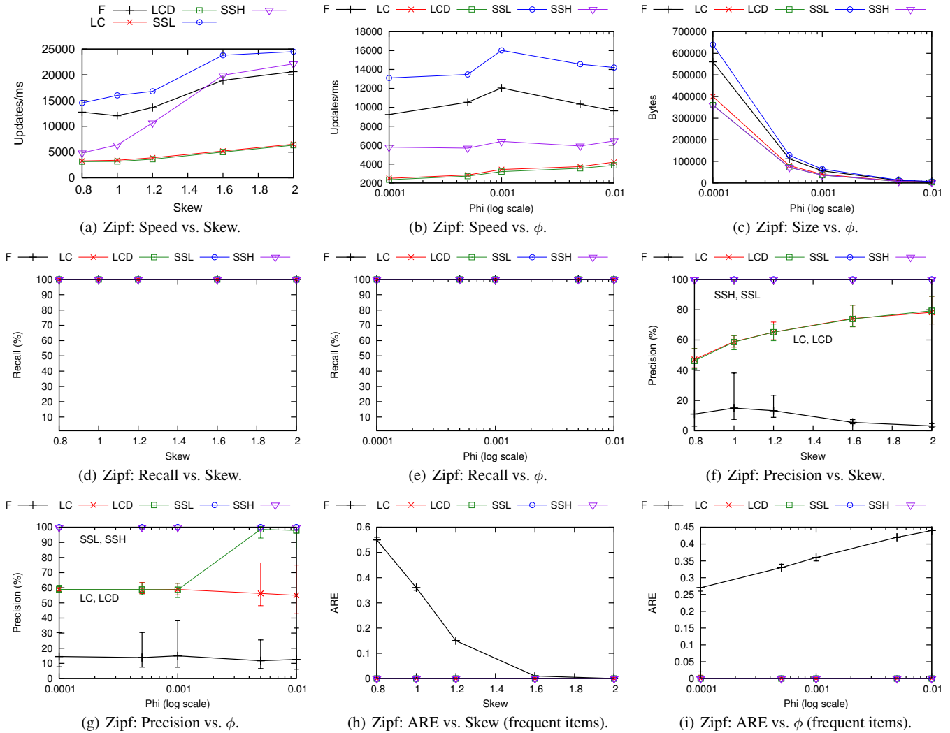
Fig. 6 Performance of counter-based algorithms on synthetic data
