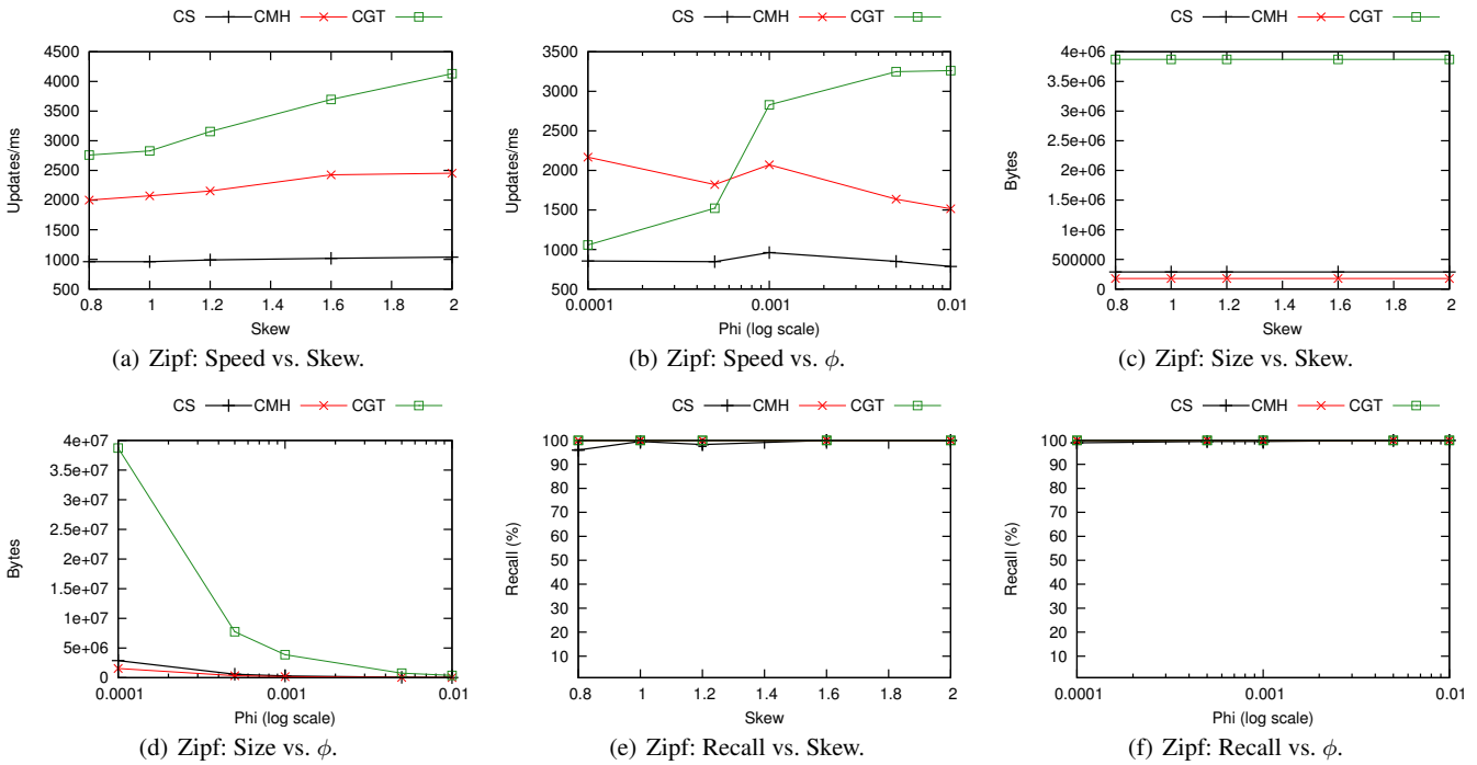
Fig. 12 Performance of sketch algorithms on synthetic data (Speed, size and recall)
