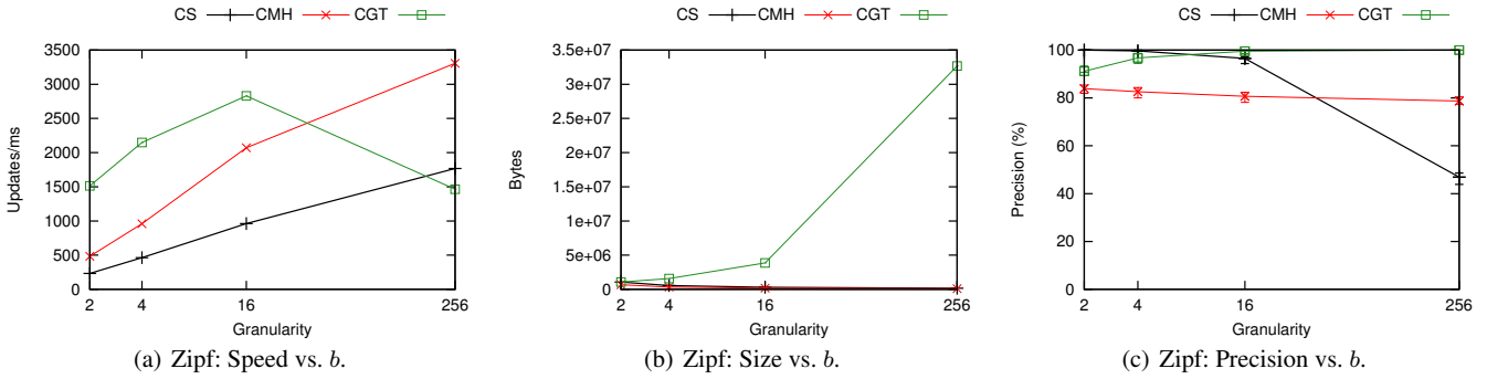
Fig. 11 Performance of sketch algorithms on synthetic data, for various granularities
