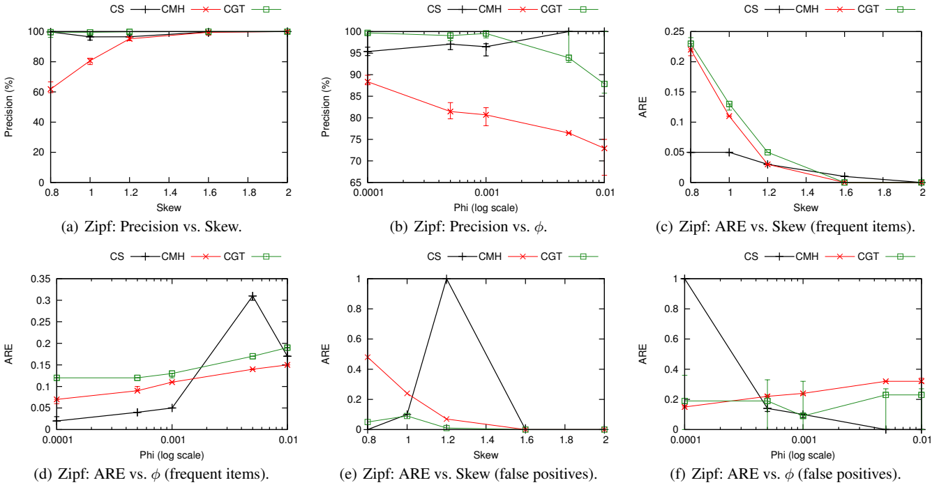
Fig. 13 Performance of sketch algorithms on synthetic data (precision and average relative error)
