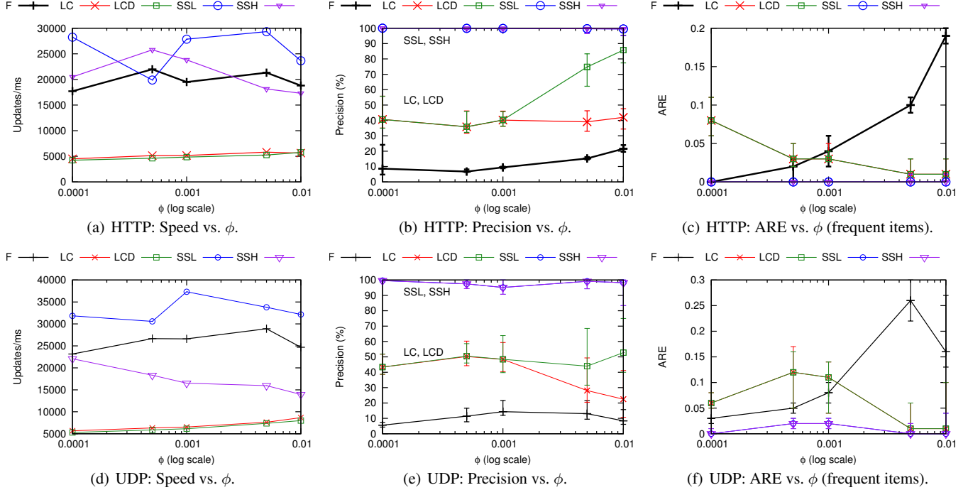
Fig. 8 Performance of counter-based algorithms on real network data
