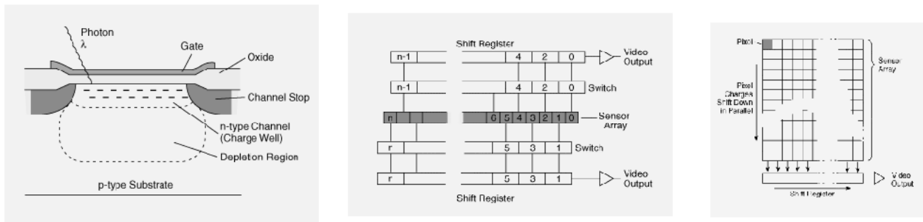
Figure 1: Operation of a CCD
