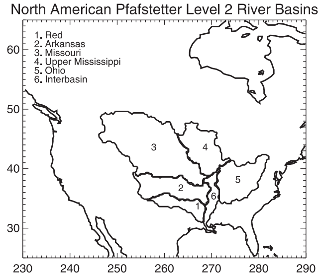
Figure 8. North American river basins.
