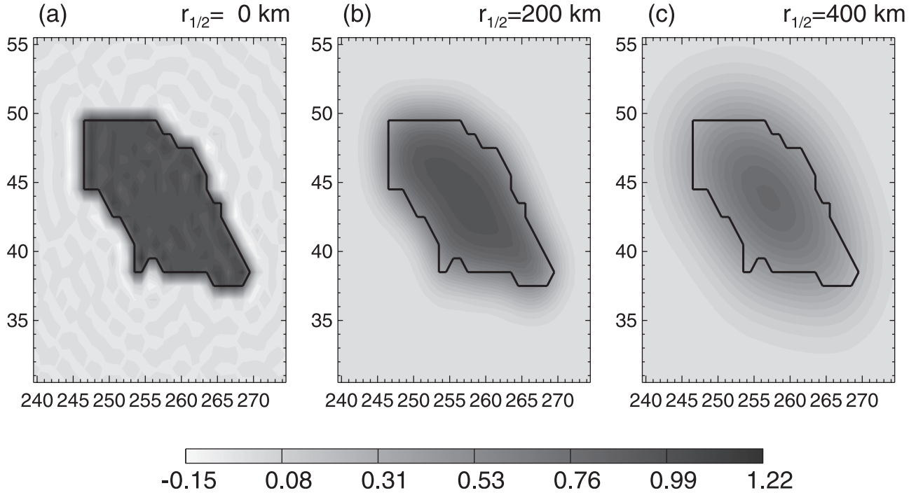
Figure 4. Examples of changing the half width of the Gaussian filter used to smooth the basin mask.
