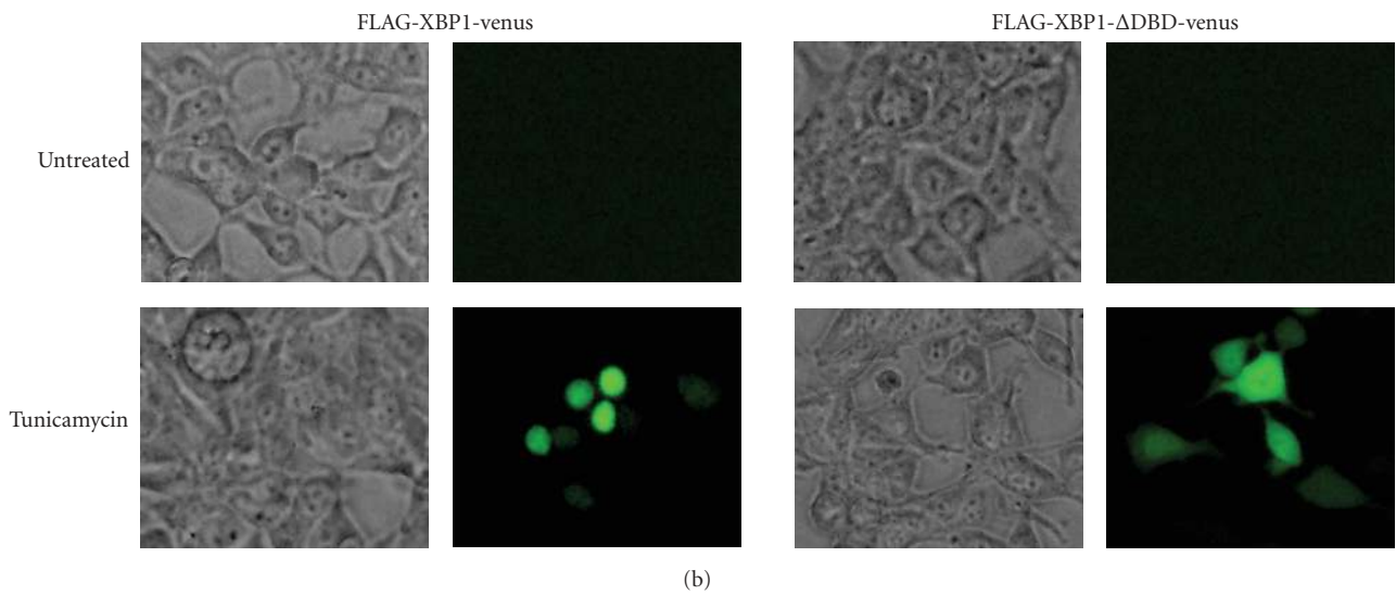
FIGURE 3: Detection of IRE1 activity using “ER stress-activated indicator” (ERAI) constructs. (a) Schematic presentation of ERAI plasmid obtained by fusing XBP1 and venus , a variant of the green fluorescent protein (adapted from [36] by Iwawaki et al. (2004)). (b) Twenty-four hours after transfection F-XBP1- venus and F-XBP1ΔDBD- venus , 293T cells were left untreated or treated with (1 μg/mL) tunicamycin for 24 hours and then analyzed by fluorescence microscopy.
